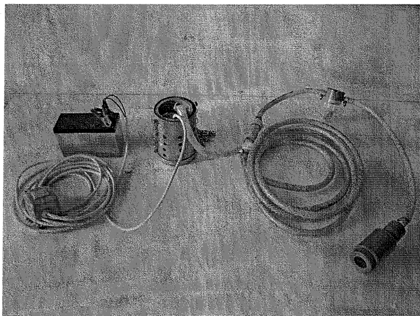
Figure 3: 'On-site' materials used to take samples from river water. From the left to the right: remote switch, battery, suction pump, tubing equipped with a 500 \mu m filter and an 80 \mu m filter, successively. The 11 \mu m pore filter is connected on the outlet pipe.
