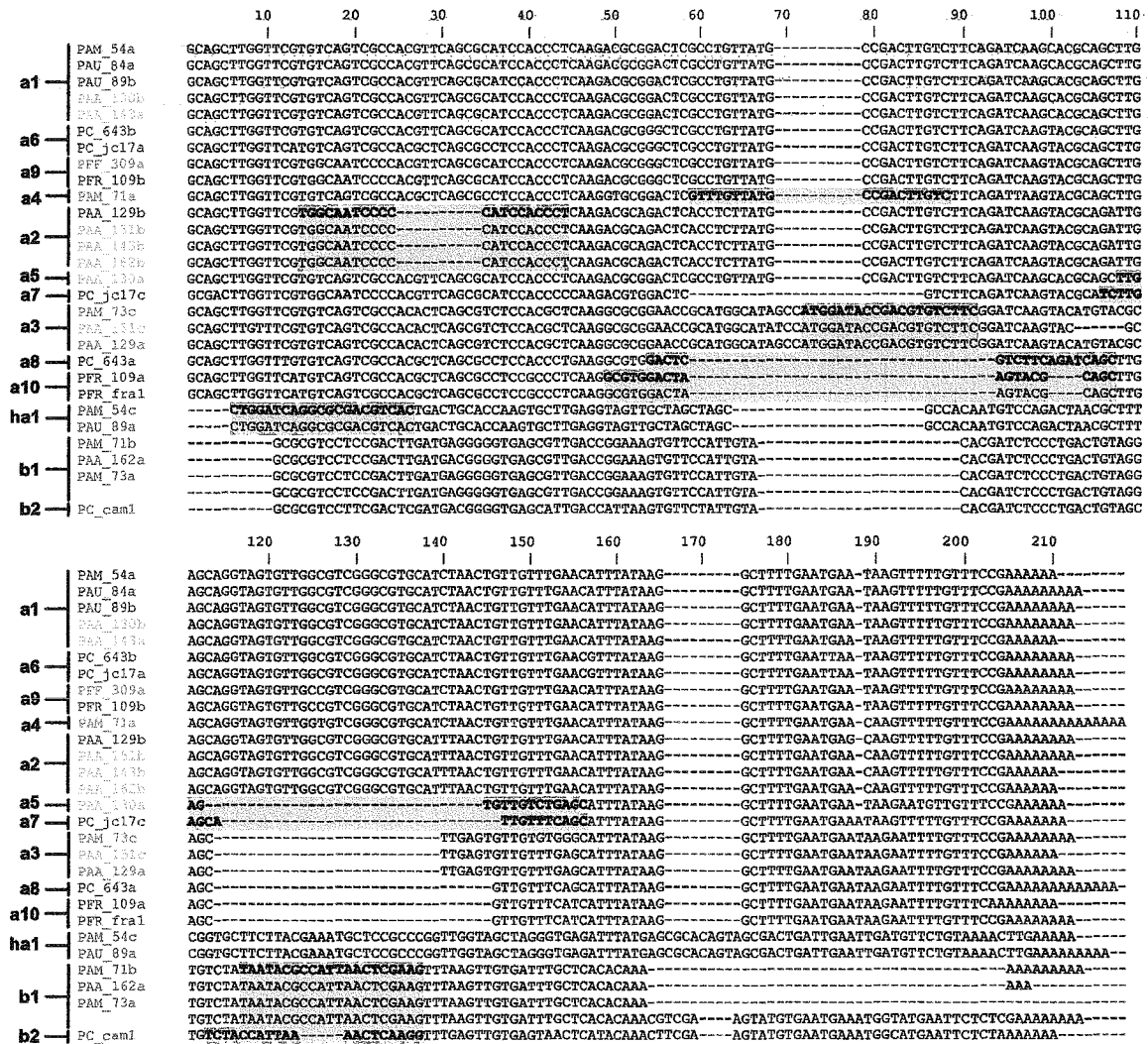
Figure 5: Sequence alignment of the region corresponding to the 3'UTR of the mRNAs, deduced from cDNA sequencing. Twenty-seven sequences obtained from our 15 isolate-panel are aligned along with 3'UTR mRNA sequences from P. fragariae var. rubi ( PFR_fra1 ) and P. cambivora ( PC_cam1 ) ( F. Panabières, unpublished data). The code of each sequence is colour-labelled according to the protein encoded: Pa_AE1.1 (red), Pa_AE1.2 (pink), Pa_AE2 (orange), Pa_BE1 (dark green), Pa_BE2 (light green), Pa_HAE1 (blue). 3'UTR specific groups are indicated on the left-hand side and correspond to the clustering of identical or nearly identical sequences. For each group, shadowed sequence represents the polymorphic region from which a 3'UTR specific primer could be designed and the bold nucleotides correspond to the primer target. PFF309b 3'UTR sequence was too divergent that it could not be properly aligned. PFF309b was therefore not represented but a specific reverse primer could be designed (a11-R).
