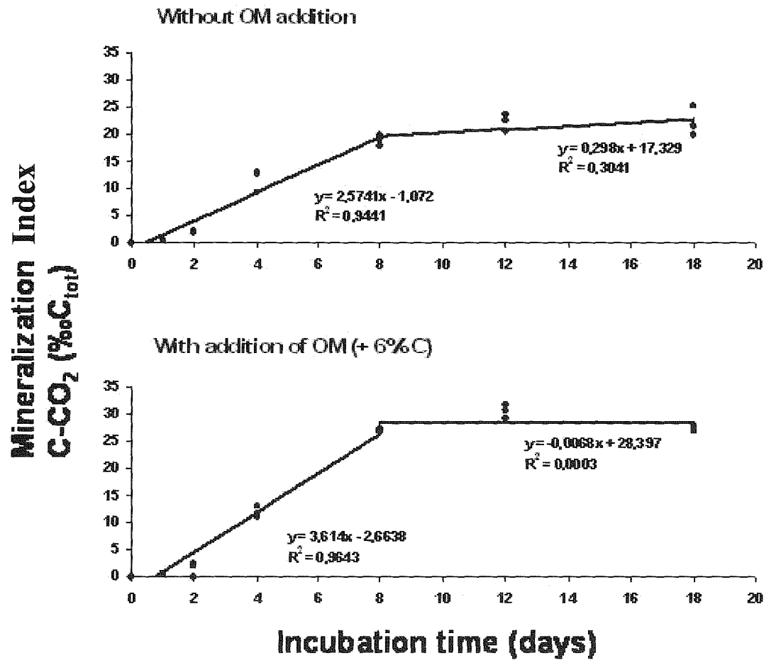
Figure 6. Cumulative organic matter mineralization after addition of WEOM ( \text{CO}_2 evolved) (mineralization index in C-CO 2 % of total organic carbon).
