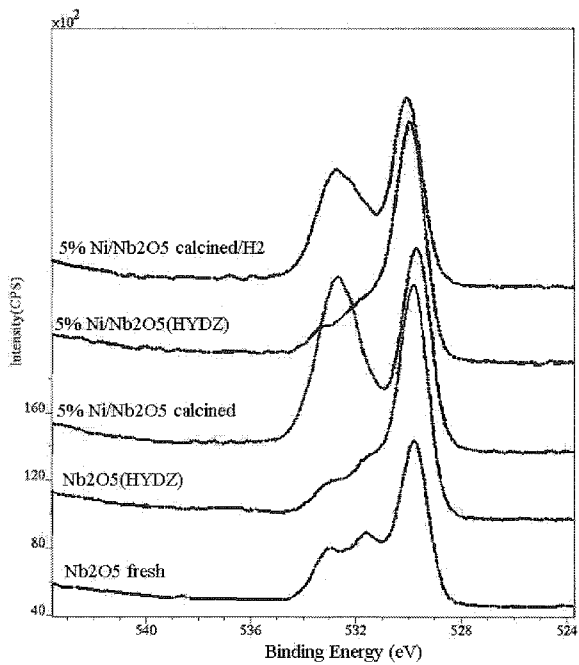
Figure IV-7. XPS spectra of the O 1s region.
