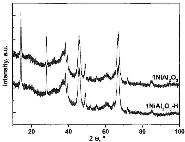
Figure III-8. XRD patterns of the nickel catalysts supported on Al 2 O 3 .
