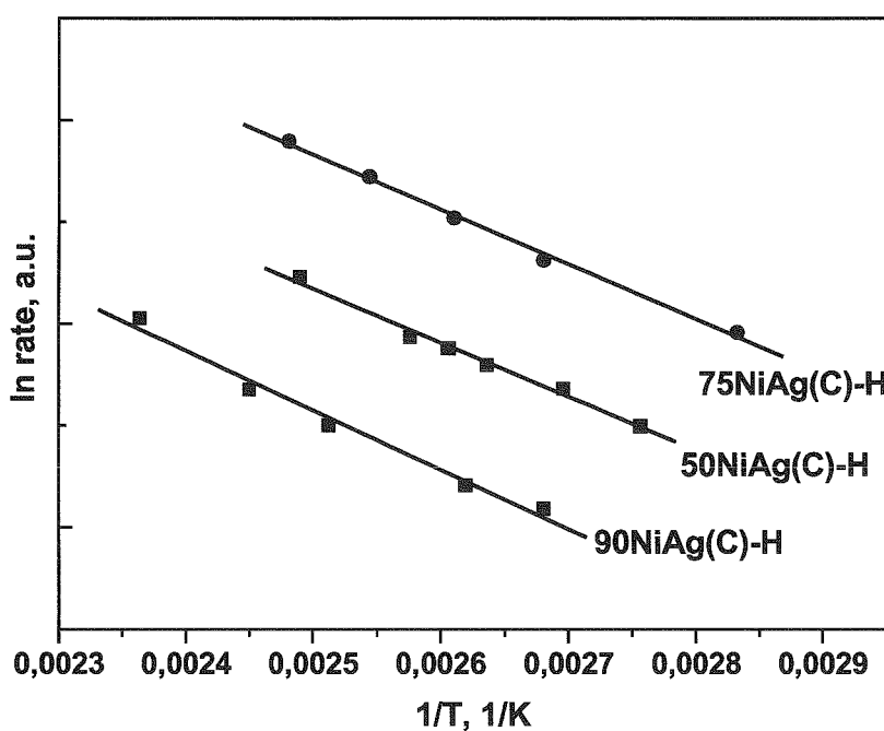
Figure VI-19. Arrhenius plots for precipitated bimetallic SiO 2 (C) catalysts.
