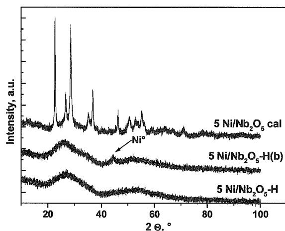
Figure IV-3. XRD patterns of the 5Ni/Nb 2 O 5 , 5Ni/Nb 2 O 5 -H and 5Ni/Nb 2 O 5 -H(b) fresh catalysts.
