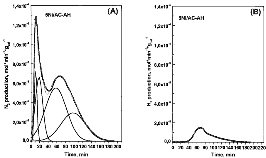
Figure VII-2. N_2 (A) and H_2 (B) emission during N_2H_4 reduction of 5Ni/AC-AH catalyst.
