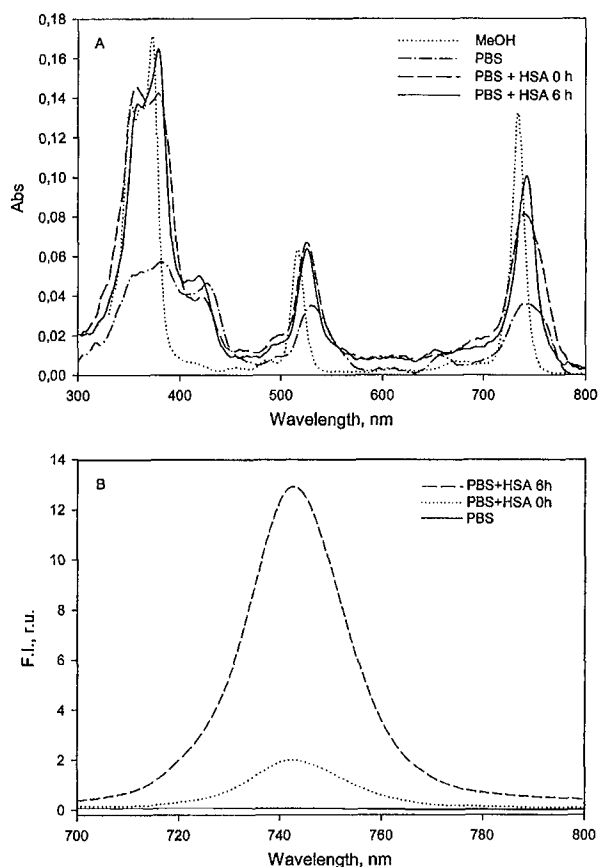
Fig. 3 Ground-state absorption spectra of m -THPBC (1.45 \mu\text{M} ) (A) in methanol ( \cdots ), PBS ( -\cdots- ) and in PBS supplemented with HSA (1 \text{mg mL}^{-1} ) with ( - ) and without incubation ( -\cdots- ). m -THPBC absorption spectra in PBS with and without HSA are magnified five times. Fluorescence spectra of 1.45 \mu\text{M} m -THPBC (B) in PBS ( - ), PBS supplemented with HSA (1 \text{mg mL}^{-1} ) with ( -\cdots- ) and without incubation ( -\cdots- ). Excitation wavelength was 378 nm.
