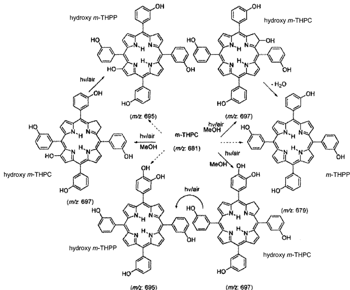
Figure 4.5. : Photooxidation products of m -THPC in methanol from (Bonnert and Martínez, 2001)
