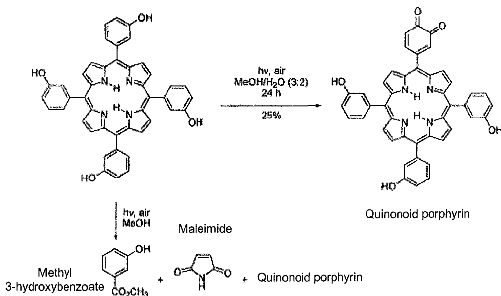
Figure 4.3. : Photoproducts formation upon light irradiation of m -THPP in methanol or methanol-water solution, from (Bonnett and Martínez, 2001).
