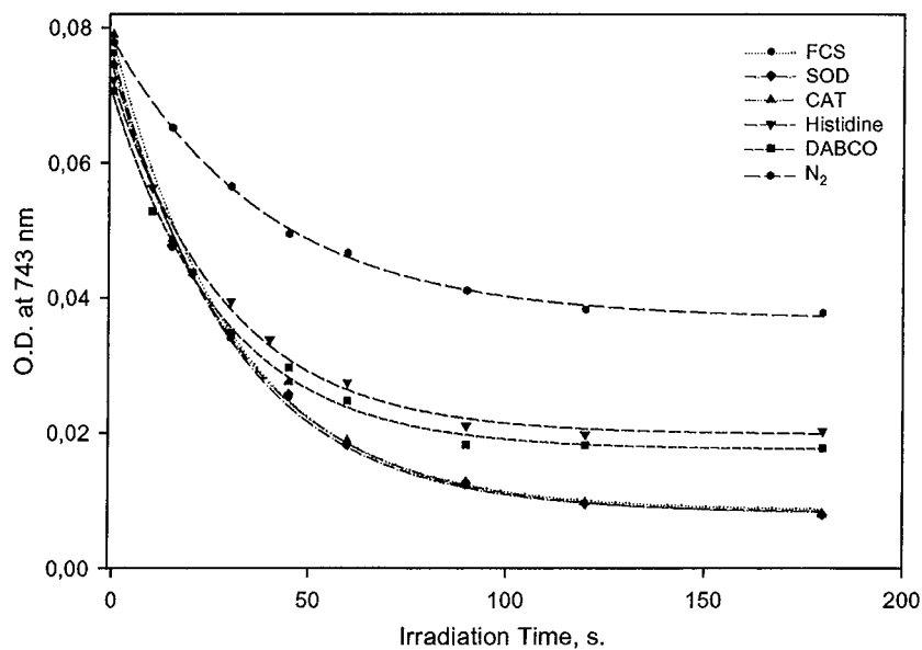
Figure 3.4. Effect of N 2 , antioxidant enzyme and singlet oxygen quenchers on the photobleaching of m-THPBC in PBS solution supplemented with 10% FCS. Histidine and DABCO were added to a final concentration of 10mM, SOD concentration was 40 \mu\text{g mL}^{-1} , and CAT concentration was 45 \mu\text{g mL}^{-1} . Bubbling with nitrogen runs during 30 min.
