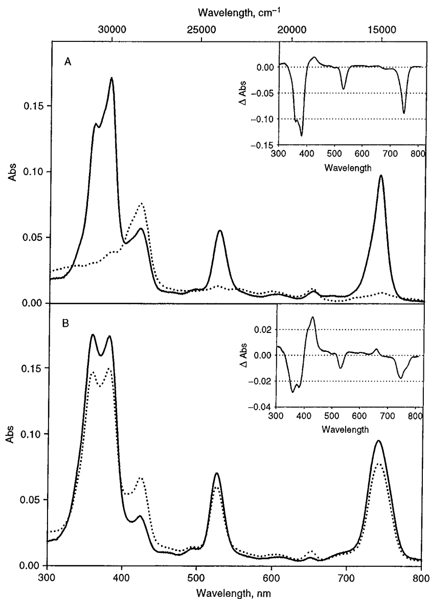
Figure 2. Absorption spectra of m -THPBC ( 10^{-5} M) before (full line), and after irradiation with 6 \text{ J cm}^{-2} at 739 \text{ nm} (dotted line). Absorption spectra of m -THPBC in HSA-PBS 6 h after incubation at 37^\circ \text{C} (A), and in freshly prepared HSA-PBS solution (B).
