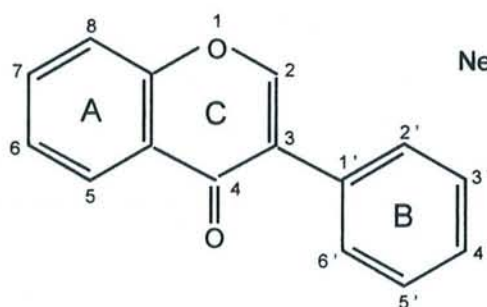
Isoflavonoid
