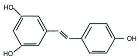
Resveratrol
