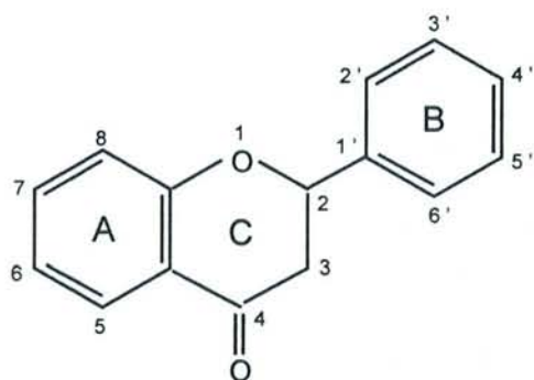
Flavonoid
