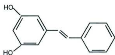
Pinosylvin
