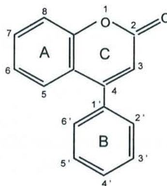
Neoflavonoid
