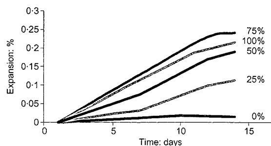
Fig. 5. Time evolution of the reactivity of the sand tested in the mixture at different percentages (RILEM TC-106 method)
