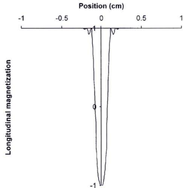
FIG. 1. Profile of the longitudinal magnetization (simulation performed according to methods developed in Ref. 4) corresponding to the application of sequence (15) with n\alpha = \pi . For this simulation, the B_1 field profile was assimilated to a Gaussian function (in view of experimental determination of the actual amplitude of B_1 along the considered axis) with a standard deviation of 1.5 mm and n was set at 64.
