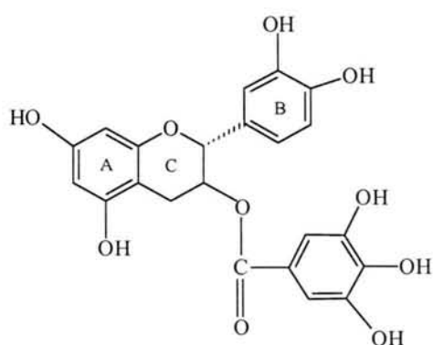
(-)-catechin gallate
