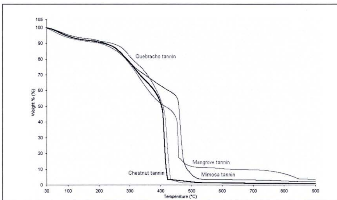
Fig. 3.5 Comparison of the thermogravimetry analysis (TGA) of mangrove tannins with the commercial mimosa, quebracho and chestnut tannins.
