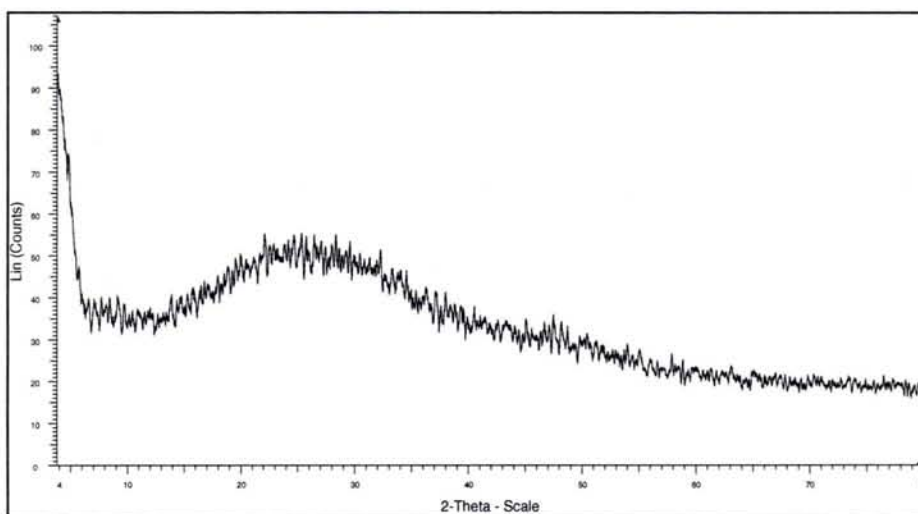
Fig. 3.26 XRD pattern of ferric-tannates synthesised at pH 3.0.
