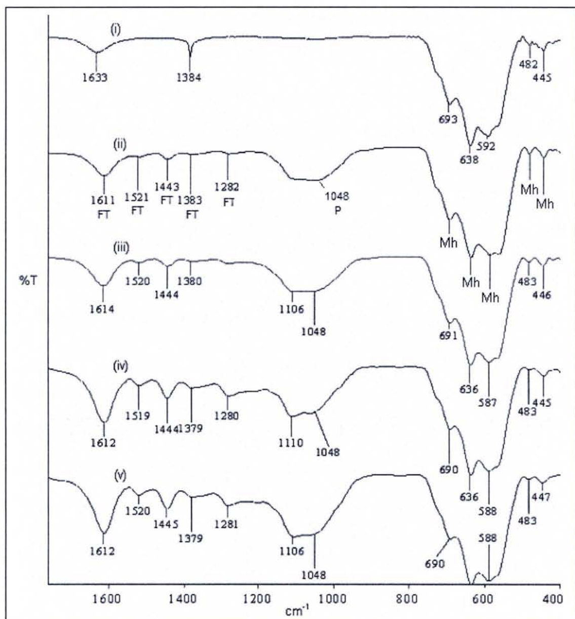
Fig. 3.76 FTIR spectrum of (i) untreated maghemite and maghemite treated with 0.5 % mangrove tannins and 15 % phosphoric acid after (ii) 1 day, (iii) 1 week, (iv) 2 weeks and (v) 1 month : FT-ferric-tannate, Mh-maghemite, P-phosphates.
