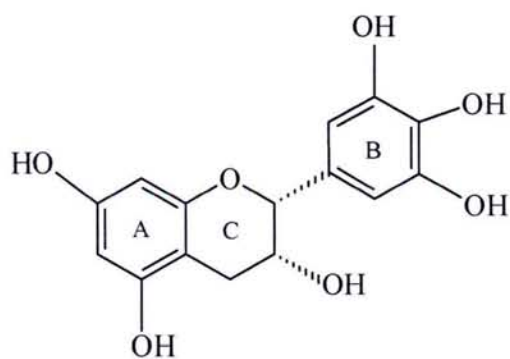
(-)-epigallocatechin
