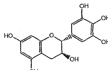
Figure 1.11 : (+)-gallocatéchine
