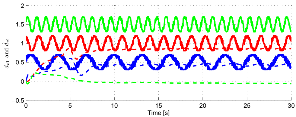
Figure 4.86: Disturbances and estimations of d_v of the leader quadrotor 1
