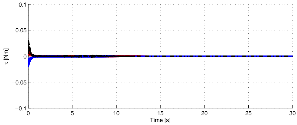
Figure 4.9: Torque of 12 quadrotors.
