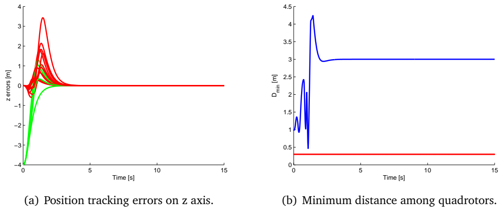
Figure 4.91: Position tracking errors on z axis and the minimum distance among quadrotors in the formation.
