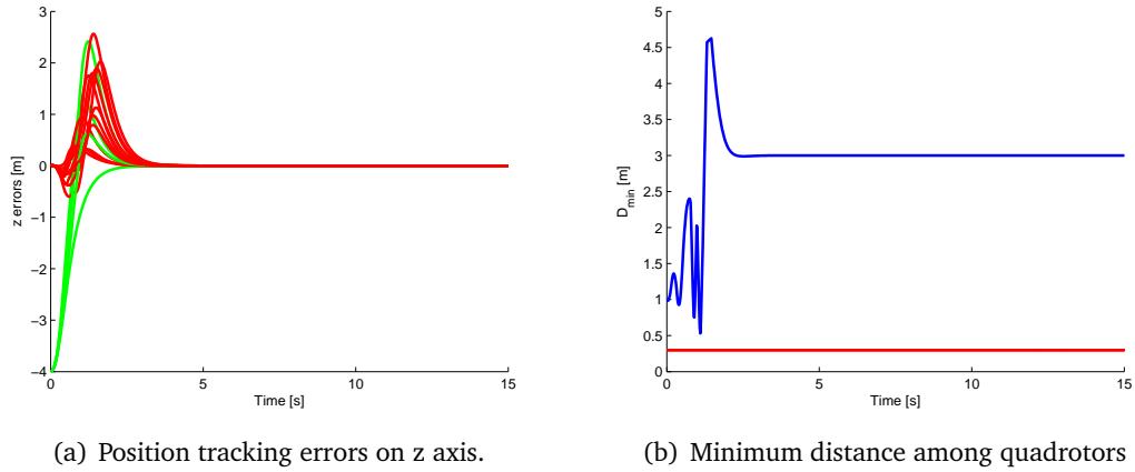
Figure 4.97: Position tracking errors on z axis and the minimum distance among quadrotors in the formation.
