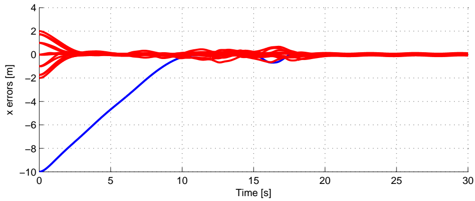
Figure 4.64: Position tracking errors on x axis.
