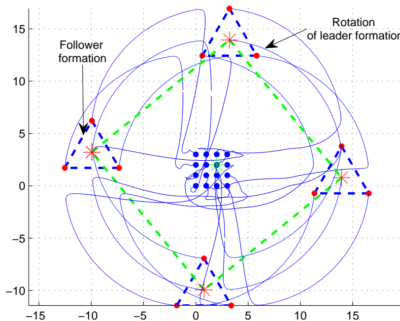
Figure 4.95: The leader-follower formation of of four leaders and three followers in each group distributed around a goal point
