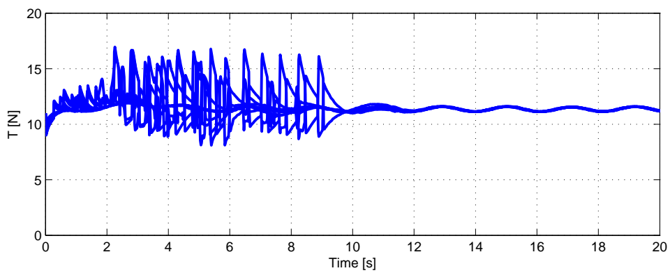
Figure 4.35: Thrust force of 9 quadrotors.
