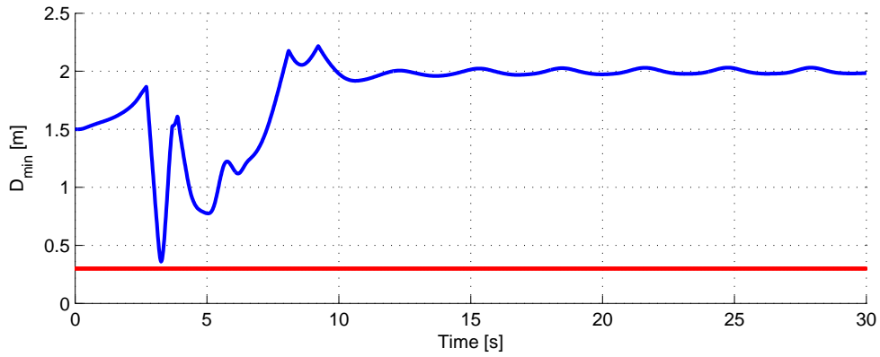
Figure 4.81: The minimum distance among quadrotors.
