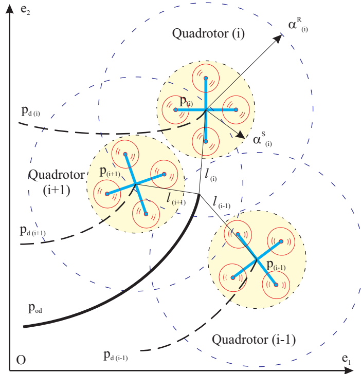
Figure 4.1: Formation parameters.
