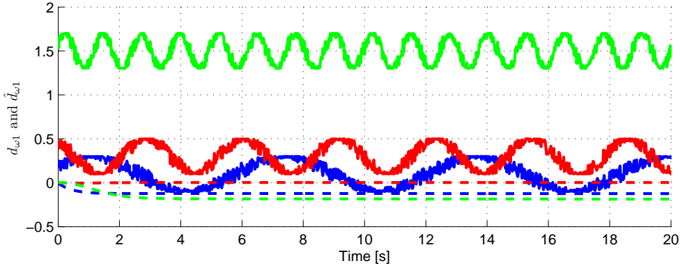
Figure 4.87: Disturbances and estimations of d_o of the leader quadrotor 1
