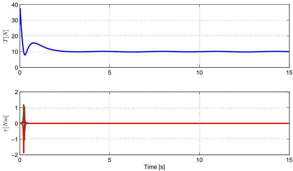
Figure 3.6: Thrust and torques.
