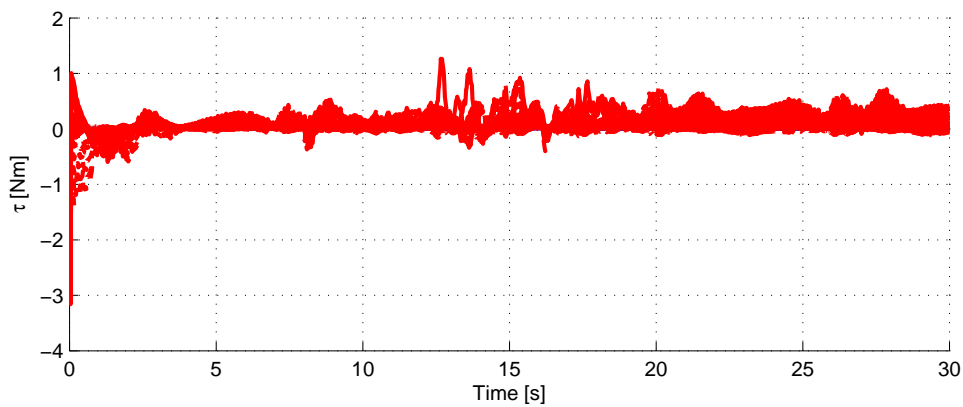
Figure 4.72: Torques of the leader and followers.
