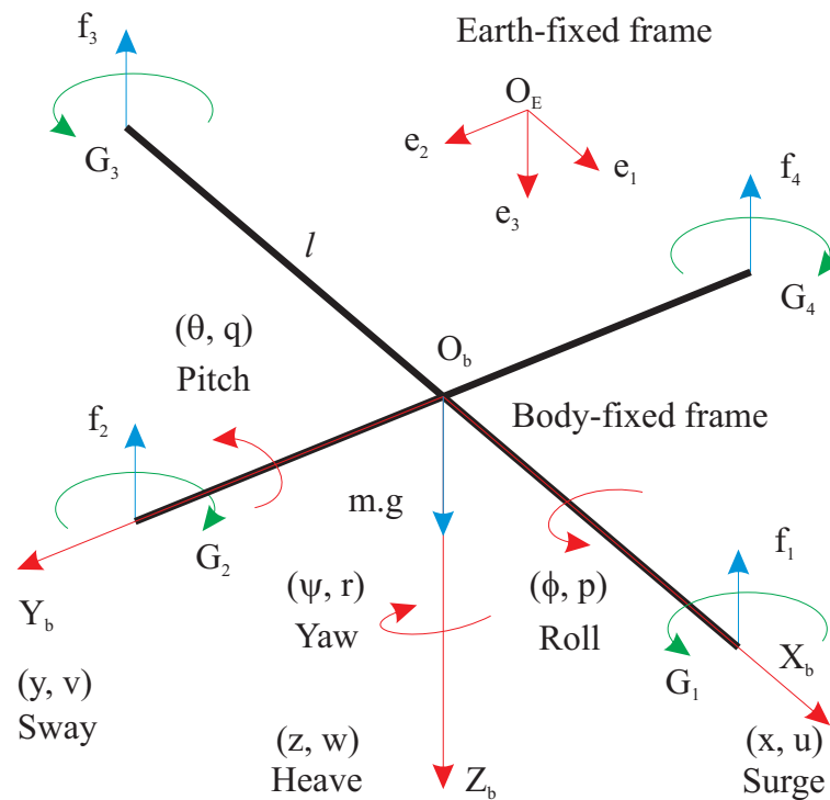
Figure 2.2: Quadrotor parameters.
