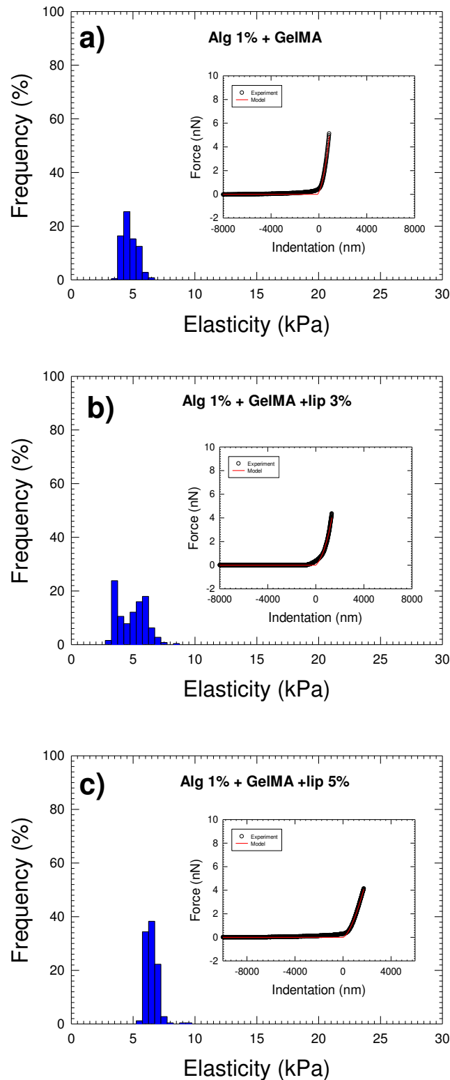
Fig.4. Statistic distribution of elastic modulus of mixed gel of GelMA and alginate at 1% before (a) and after liposomes blending at 3% (b) and 5% (c). The inset corresponds to experimental force curve (white circle) and theoretical fitting (red line) for the most frequent elastic modulus value. Each distribution derived from the fitting of 1024 force curves.
