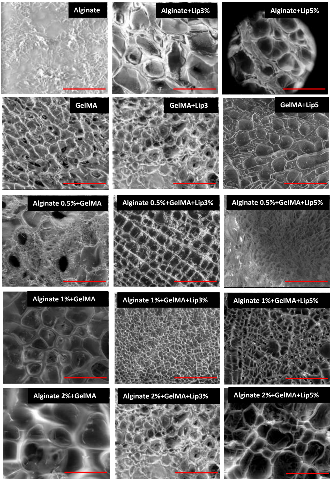
Fig.2. SEM images of 3D hydrogels of various systems before and after functionalization (scale bar is 300 μm).
