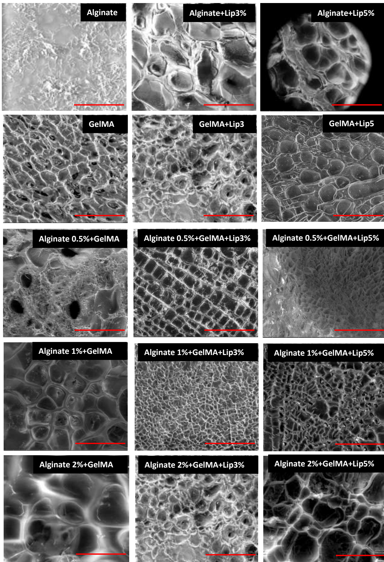
Fig.2. SEM images of 3D hydrogels of various systems before and after functionalization (scale bar is 300 \mu m).
