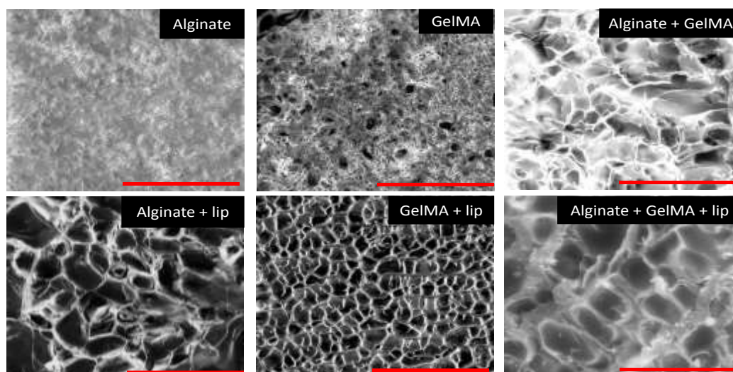
Fig.2. SEM micrographs of alginate, GelMA and alginate/GelMA IPN hydrogels with and without nanoliposomes (scale bar is 300 µm).
