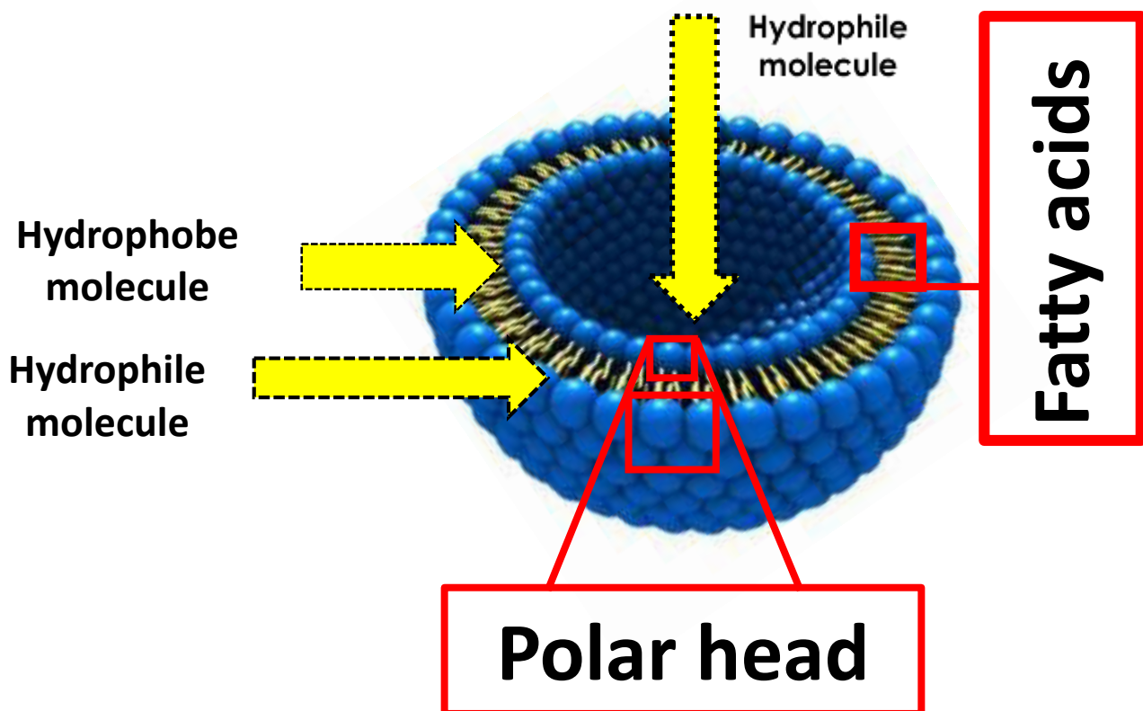
Fig.9. Structure of liposomes, organized in bilayer with hydrophilic polar heads and hydrophobic apolar tails.
