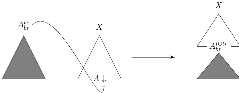
Figure 3.8: Feature Unification during Substitution in FB-LTAG
