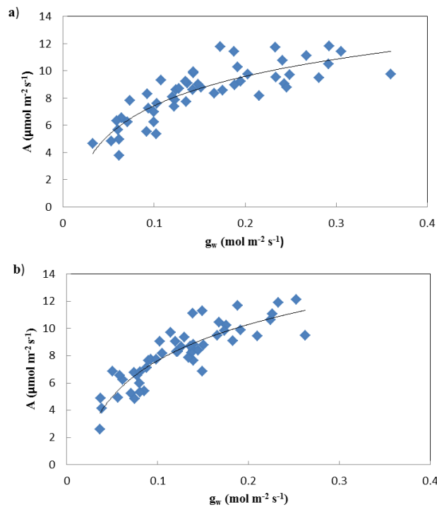
Figure 3 Relationships between net \text{CO}_2 assimilation ( A ) and stomatal conductance ( g_w ) at a) low VPD_L , b) high VPD_L . Each point represents one leaf sampled on 5 trees from each of the 10 clones.
