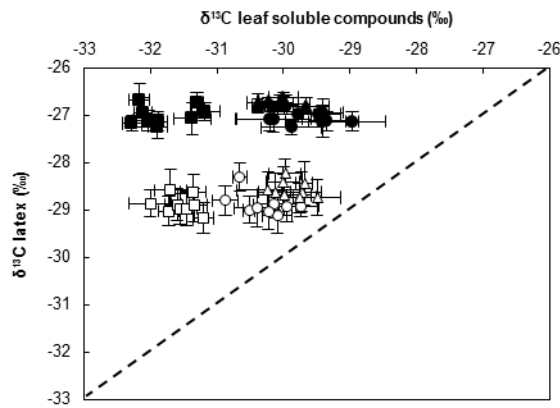
Figure 16 Relationship between carbon isotope composition of latex ( \delta^{13}\text{C-L} ) and of leaf soluble compounds ( \delta^{13}\text{C-S} ) in August 2013 (squares), November 2013 (circles) and April 2014 (triangles) in tapped (open symbols) and untapped (closed symbols) twenty-year old rubber trees. Each value is daily average (with standard error) of 10 (2 sampling times \times 5 trees) replicates for leaf soluble compounds and 25 (5 sampling times \times 5 trees) replicates for trunk latex collected on 5 trees.
