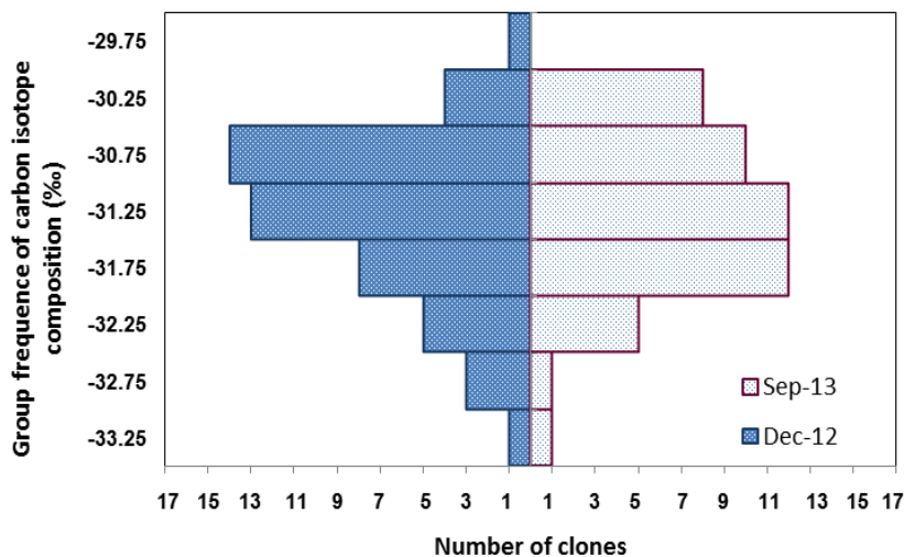
Figure 8 Frequency distribution of carbon isotope composition in bulk leaf ( \delta^{13}\text{C} ) in the dry season (December, left) and in the rainy season (September, right). N=49.
