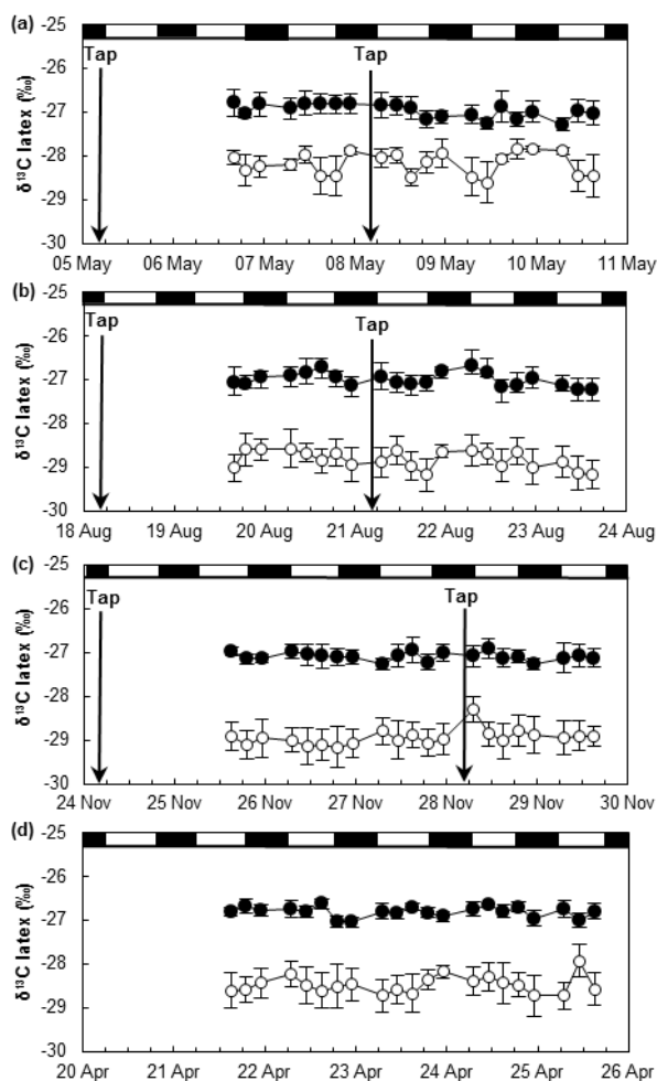
Figure 15 Mean carbon isotope composition of trunk latex ( \delta^{13}\text{C-L} ) over the courses of five-day sampling periods in a) May 2013, b) August 2013, c) November 2013 and d) April 2014 in tapped (open symbols, dashed lines) and untapped (closed symbols, solid line) twenty-year old rubber trees. Each value is an average (with standard error) of samples collected on 5 trees. The vertical arrows show the tapping times.
