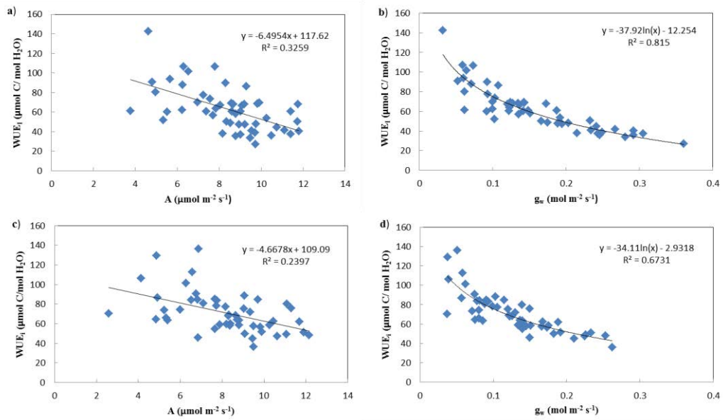
Figure 4 Relationships between intrinsic water use efficiency ( WUE_i ) and net \text{CO}_2 assimilation ( A ) at a) low VPD_L , c) high VPD_L , and relationships between intrinsic water use efficiency ( WUE_i ) and stomatal conductance ( g_w ) at b) low VPD_L , d) high VPD_L . Each point represents one leaf sampled on 5 trees from each of the 10 clones.
