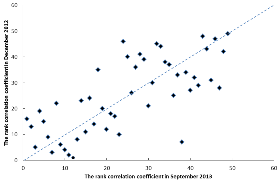
Figure 9 Relation between the genotype ranking based on \delta^{13}\text{C} values measured on the 49 genotypes in the dry season (December 2012) and wet season (September 2013). Each point represents a clone. The dotted line represents the 1/1 line. The Spearman rank correlation coefficient was 0.72.
