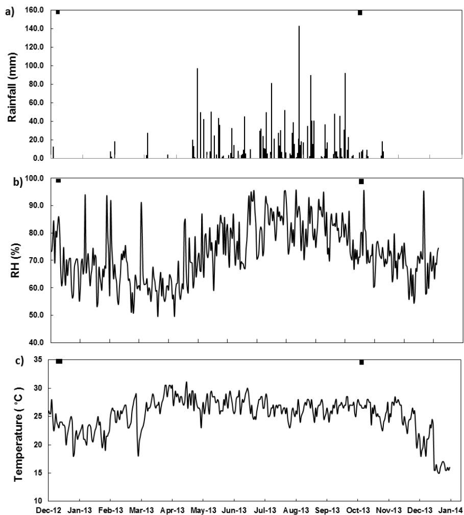
Figure 7 Annual courses of a) daily rainfall, b) mean daily air humidity and c) mean daily air temperature.
