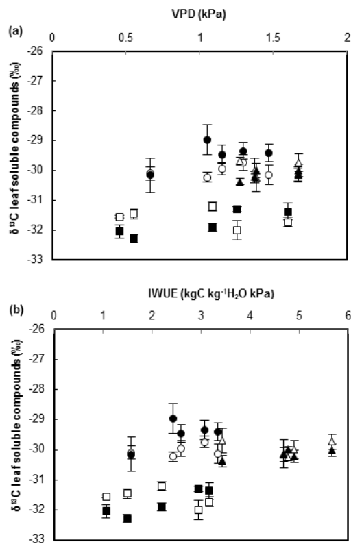
Figure 14 Relationships between carbon isotope composition of leaf soluble compounds ( \delta^{13}\text{C-S} ) and a) mean daylight vapour pressure deficit (VPD), b) inherent water-use efficiency at the ecosystem level (IWUE) in August 2013 (squares), November 2013 (circles) and April 2014 (triangles) for tapped (open symbols) and untapped (closed symbols) twenty-year old rubber trees. For \delta^{13}\text{C-S} , each value is a daily average (with standard error) of samples collected at 15:00 on 5 trees.
