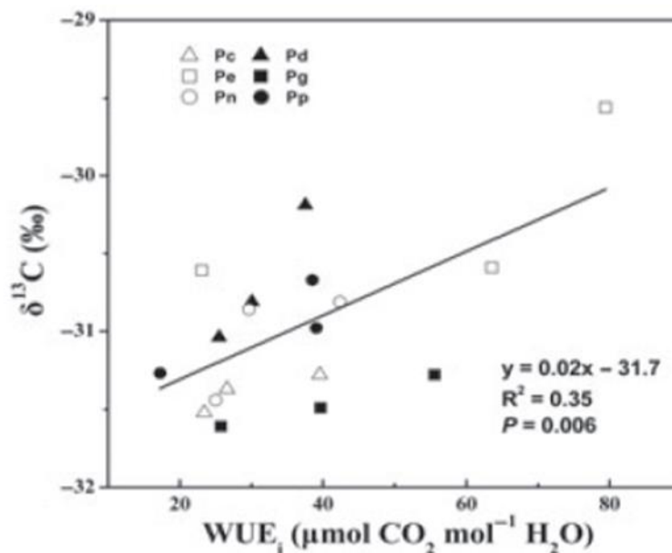
Figure 1 Carbon isotope composition (‰, \delta^{13}C ) and intrinsic water use efficiency ( WUE_i ) for P. cathayana (Pc), P. deltoides (Pd), P. euramericana (Pe), P. alba × P. glandulosa (Pg), P. nigra (Pn) and P. popularis (Pp) (Cao et al. , 2011).
