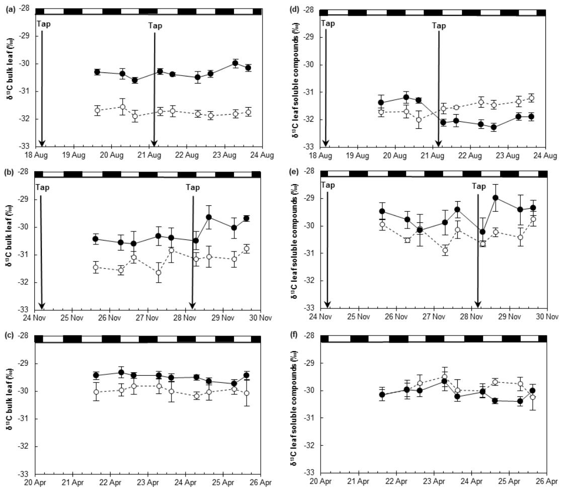
Figure 13 Mean carbon isotope composition of (a,b,c) bulk leaf ( \delta^{13}\text{C-B} ) and (d,e,f) leaf soluble compounds ( \delta^{13}\text{C-S} ) over the courses of five-day sampling periods in (a,d) August 2013, (b,e) November 2013 and (c,f) April 2014 for tapped (open symbols, dashed line) and untapped (closed symbols, solid line) twenty-year old rubber trees. Each value is an average (with standard error) of samples collected on 5 trees. The vertical arrows show the tapping times. Leaves were not collected in May 2013.
