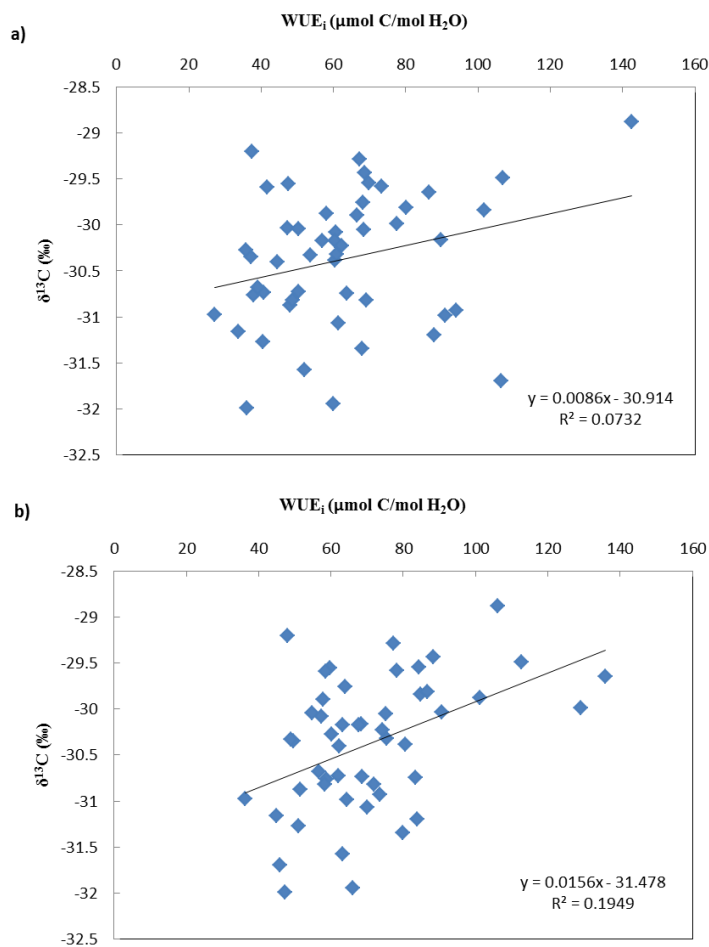
Figure 5 The relation between intrinsic water use efficiency ( WUE_i ), leaf carbon isotope composition ( \delta^{13}C ), a) low VPD_L and b) high VPD_L . Each point represents one leaf sampled on 5 trees from each of the 10 clones.
