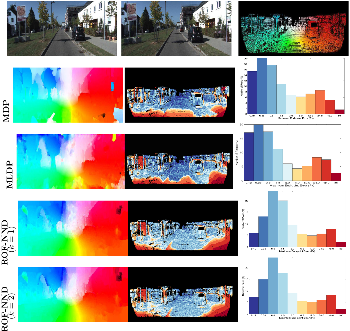
Figure 4.11: Results obtained for sequence 144 of the KITTI training datasets. First row from the top: two images for which the optical flow has to be determined with known ground truth flow on the right. Second row: results obtained for the MDP-flow2 method [Xu et al., 2012] (on the right: flow field with its usual color code, in the middle: end point error image with small and large values in blue and red respectively, on the right: bar chart of the end point errors in pixels). Third row : same results for the MLDP method [Mohamed et al., 2014]. Fourth row: results for the proposed ROF-NND method with k = 1 . Fifth row : results for the ROF-NND method with k = 2 .
