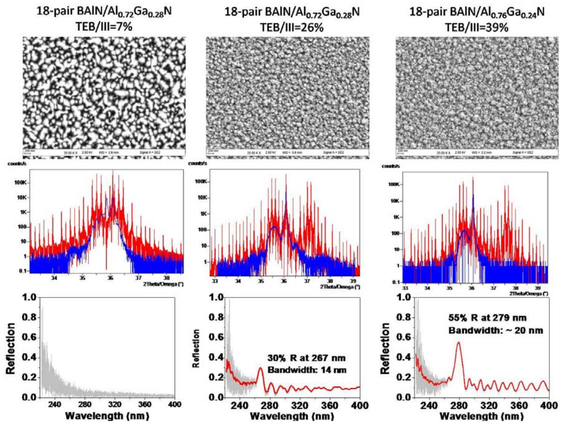
Figure 65: 18-pair BAIN/Al 0.72-0.76 Ga 0.28-0.24 N DBRs with different TEB/III ratios (The composition of boron used in the XRD fittings is estimated by an assumption that it has a linear relationship with TEB/III ratio, and it is 15% for TEB/III=39% according to EDX measurements).
