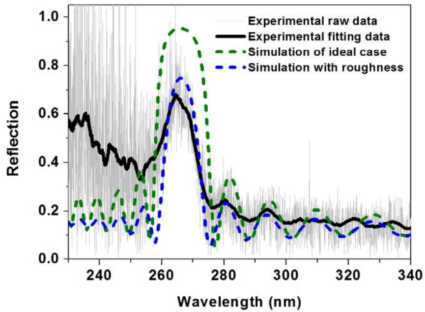
Figure 71: Comparison between experimental reflection spectrum and simulations of 18-pair BAlN/AlGaIn DBR reflecting at 265 nm.
