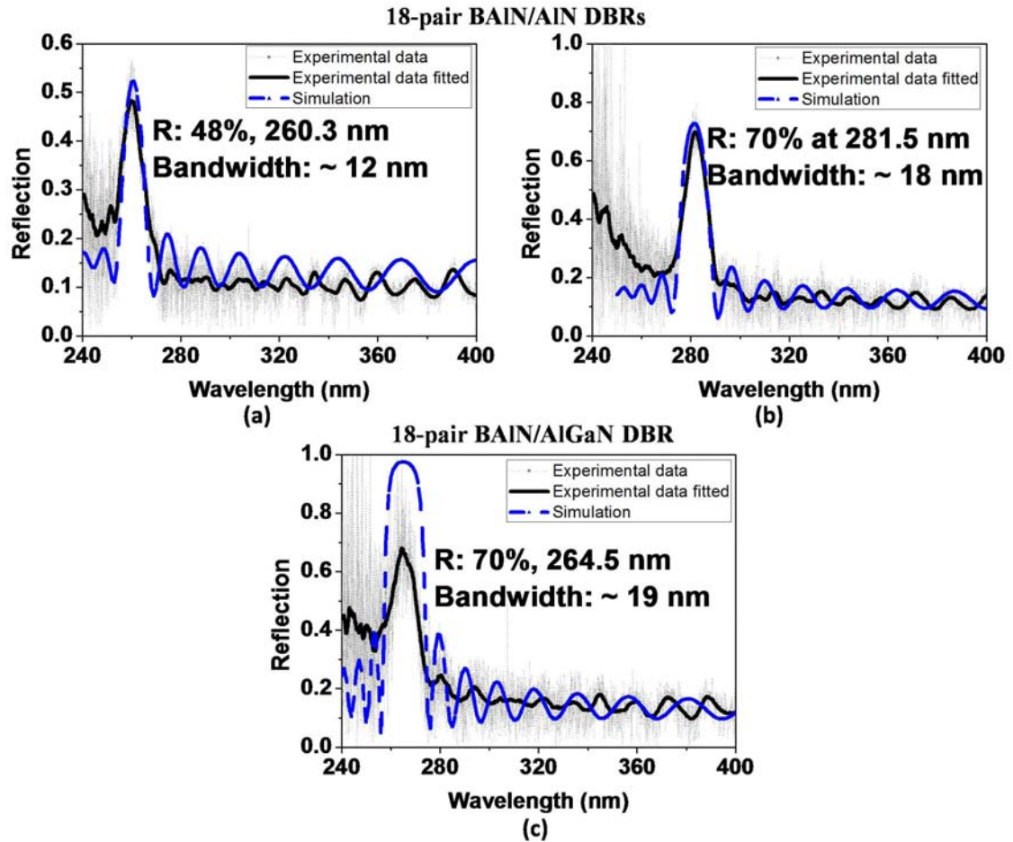
Figure 66: (a) 18-pair BAIN (29 nm) / AiN (29 nm) DBRs reflecting at 260 nm; (b) 18-pair BAIN (33 nm) / AiN (32 nm) DBRs reflecting at 280 nm; (c) 18-pair BAIN (33 nm) / Al 0.8 Ga 0.2 N (24 nm) DBRs reflecting at 265 nm.
