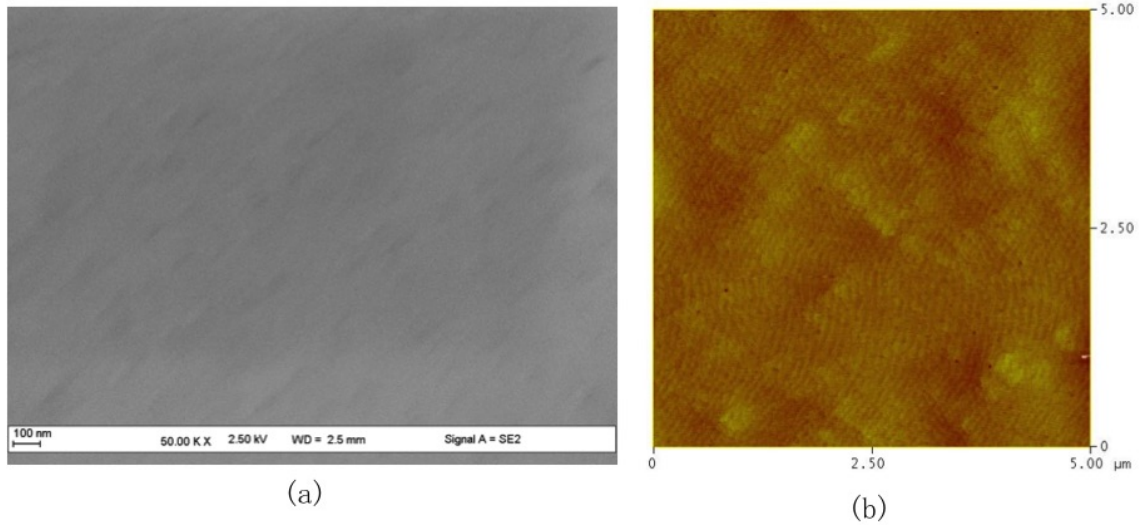
Figure 72: (a) SEM image and (b) AFM image of AlN template grown on sapphire in CCS reactor.
