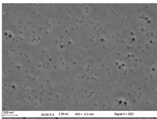
(a) 30 nm \text{Al}_{0.82}\text{Ga}_{0.18}\text{N} on AlN template
