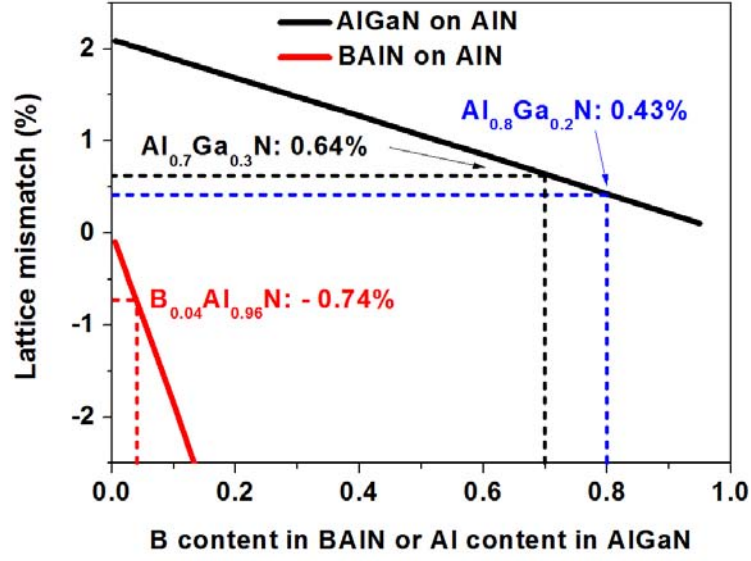
Figure 59: Lattice mismatch of AlGaN/AlN and BAlN/AlN.
