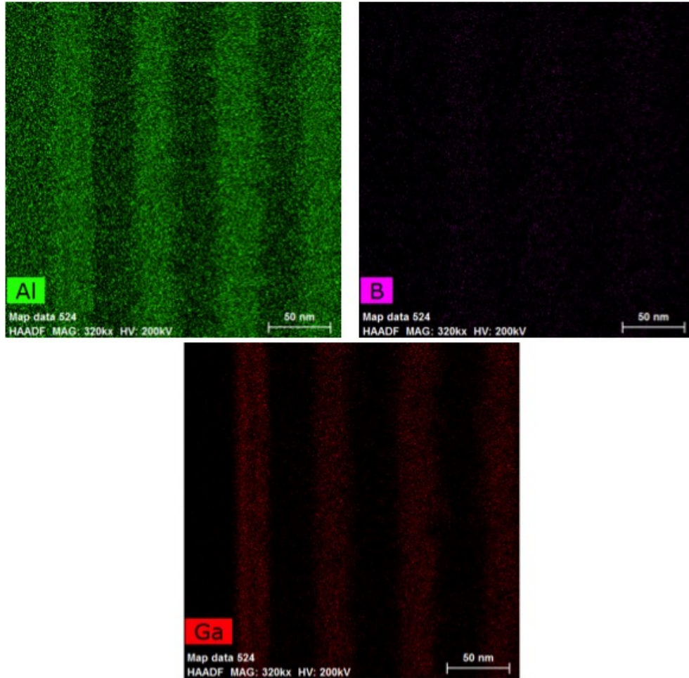
Figure 68: Cross-sectional EDX mapping of 18-pair BAlN/AlGaN DBR reflecting at 265 nm.
