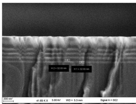
(c) 5-period AlN (30 nm) / \text{Al}_{0.82}\text{Ga}_{0.18}\text{N} (30 nm) on AlN template (cross-section)
