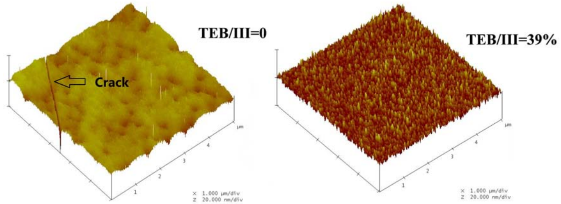
Figure 32: AFM images of 40 nm BAIN layers grown on GaN templates under TEB/III ratio of 0% and 39%.
