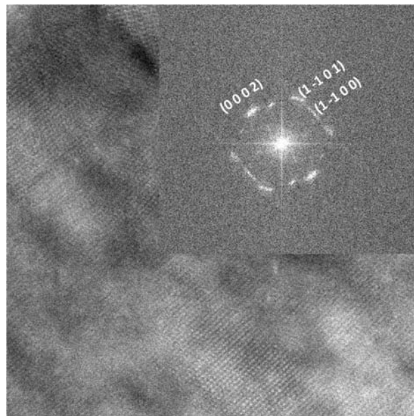
Figure 36: Cross section High-angle Annular Dark Field Scanning Transmission Microscopy (HAADF-STEM) image of 75 nm BAIN layer containing 12% boron; inset shows diffraction pattern after Fast Fourier Transform (FFT).
