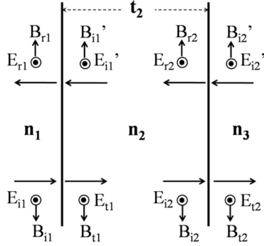
Figure 55: Schematic of electromagnetic wave propagation in the DBR structure.
