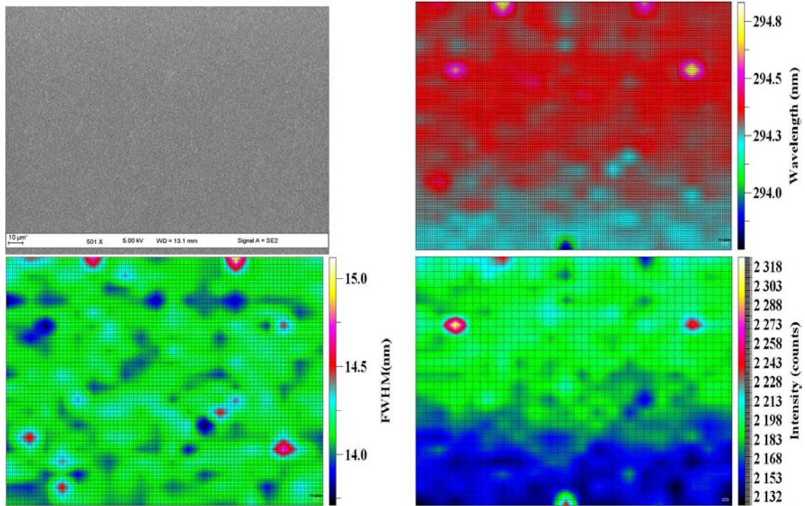
Figure 48: CL hyperspectral mapping of 20-period MQWs at room temperature.
