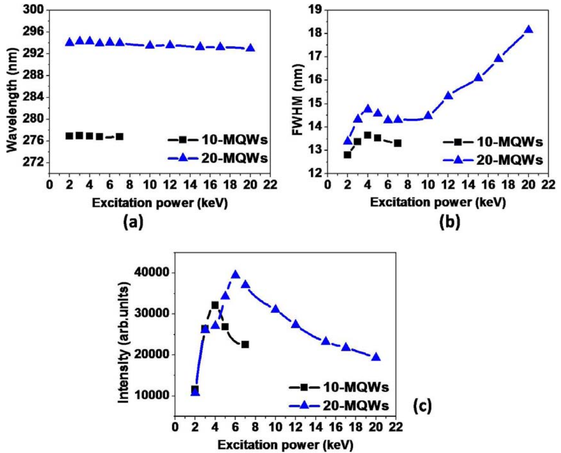
Figure 47: Comparison of (a) CL emission wavelength, (b) FWHM and (c) emission intensity at room temperature between 10- and 20-period MQWs grown on a relaxed AlGaIn buffer on AlN templates.
