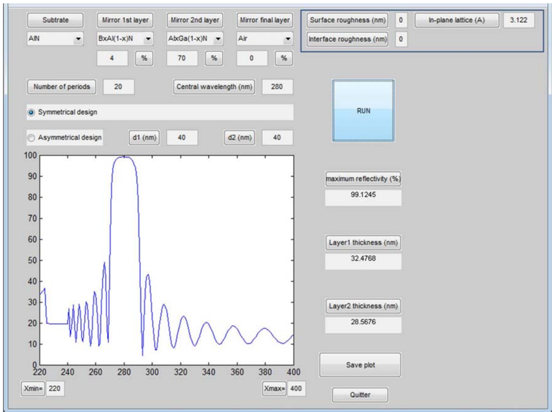
Figure 62: Reflector software interface with factors of surface roughness, interface roughness and strain.
