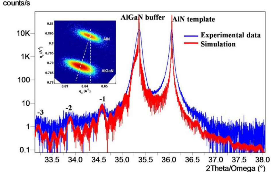
Figure 41: (0 0 0 2) 2\theta - \omega scan for 4 quantum wells grown on a relaxed buffer on AlN template and the simulation of the structure which used values obtained by XRD, STEM and EDX analyses. The RSM of (1 1 -2 4) reflection is shown in the inset.
