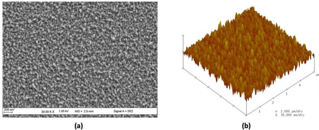
Figure 26: (a) SEM and (b) AFM images of 5-period AlN/BAlN heterostructure (310 nm for total thickness).
