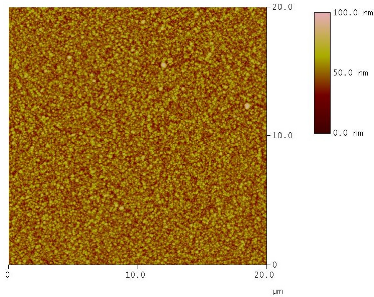
Figure 70: AFM image of 18-pair BAlN/AlGaN DBR reflecting at 265 nm.
