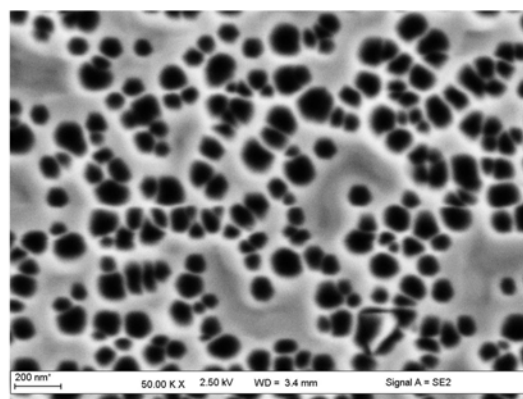
(b) 5-period AlN (30 nm) / \text{Al}_{0.82}\text{Ga}_{0.18}\text{N} (30 nm) on AlN template
