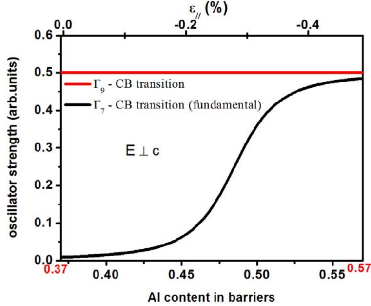
Figure 39: Relative oscillator strengths for the optical transitions between the valence bands ( \Gamma_7 (CH) and \Gamma_9 (HH)) and conduction band (CB) in an AlGa N /AlGa N quantum well as a function of the Al composition in the barriers, with Al content in the well fixed to x_{Al} = 0.37 . The corresponding strain in the well is also reported in the top axis. Calculations consider that the barriers are strain-free and QWs are fully-strained on AlGa N barriers.
