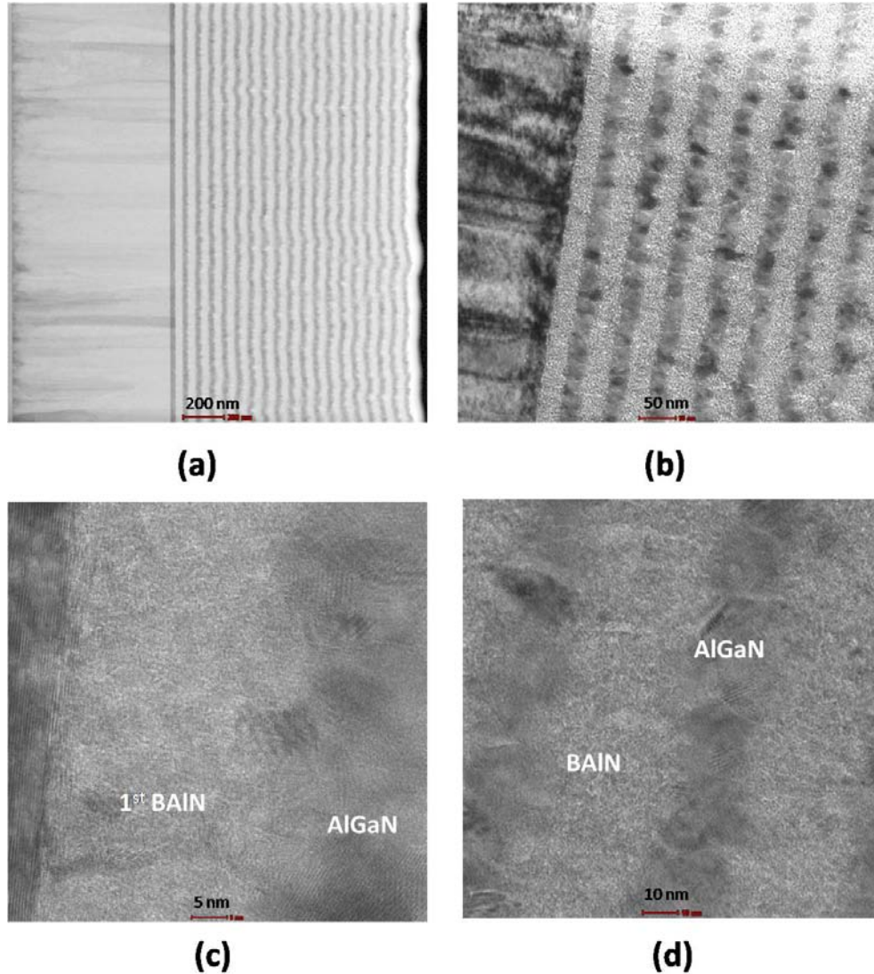
Figure 67: (a) HAADF-STEM (BF) image of 18-pair BAIN/ \text{Al}_{0.8}\text{Ga}_{0.2}\text{N} DBRs reflecting at 265 nm. (b), (c) and (d) are TEM images with different magnifications.
