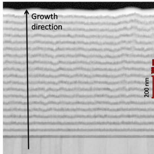
(a) 18-period BAlN (32 nm)/AlGaIn (24 nm) grown at 1000 °C in a continuous way
