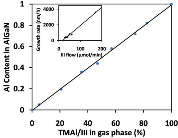
Figure 15: Al composition of AlGaN layers fully-strained on AlN templates versus TMAI/III ratio. The inset shows the growth rate versus total flow rate of (TMAI+TMG).
