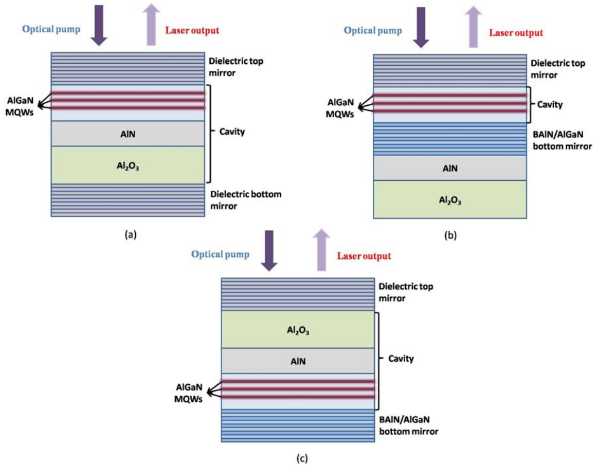
Figure 73: (a) VCSEL design with dielectric top and bottom mirrors; (b) VCSEL design with dielectric top mirror and BAIN/AlGaIn bottom mirror; (c) inverted VCSEL structure with BAIN/AlGaIn bottom mirror grown on the active region.
