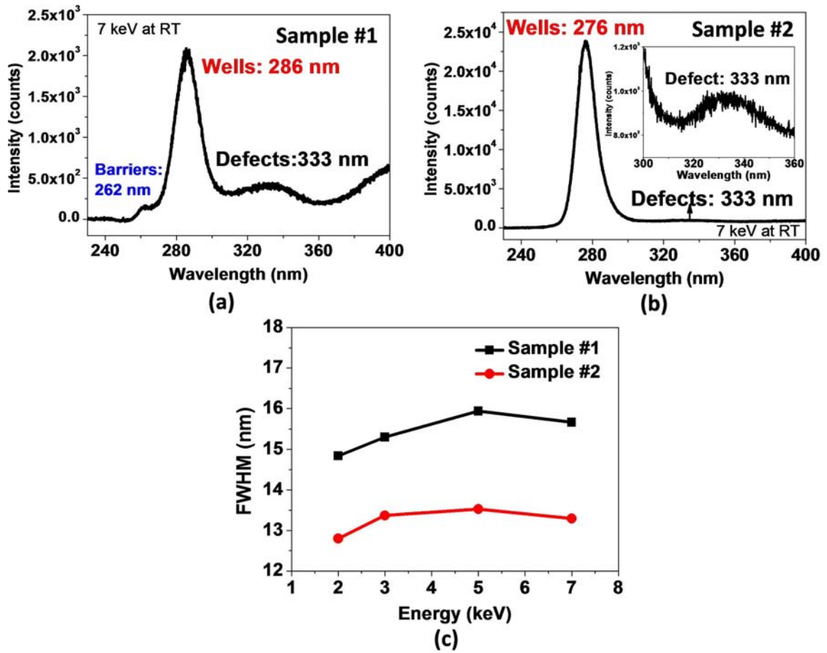
Figure 54: CL spectra under 7 keV at room temperature for (a) sample #1 and (b) sample #2; (c) is FWHM of QW emission peaks under different electron beam energies at room temperature.
