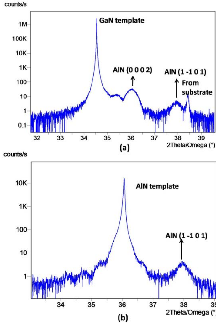
Figure 25: HR-XRD 2\theta - \omega scans of 5-period AlN/BAlN heterostructure grown on (a) GaN template and (b) AlN template.
