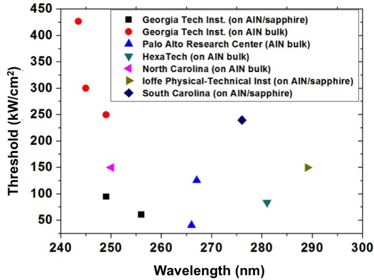
Figure 6: State-of-the-art optically-pumped AlGaN DUV lasers.
