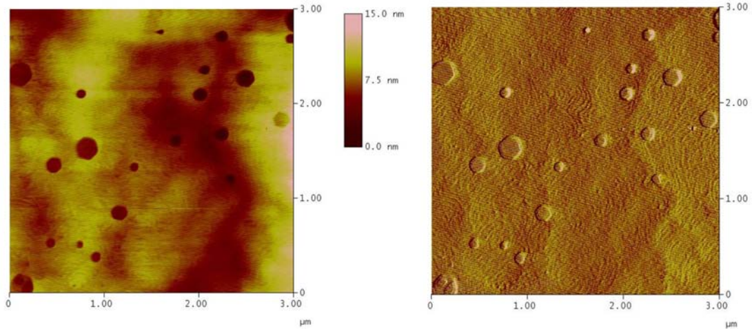
Figure 45: AFM images of 20-period MQWs grown on a relaxed AlGaIn buffer on AlN templates.
