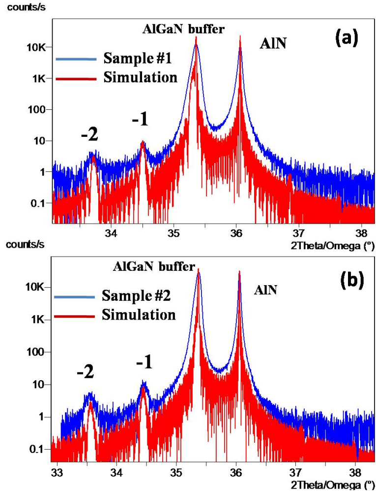
Figure 49: 2\theta - \omega scans of (a) sample #1 and (b) sample #2.
