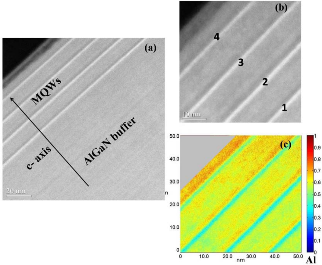
Figure 42: (a) Cross-section High-angle Annular Dark Field Scanning Transmission Electron Microscopy (HAADF-STEM) images taken along \langle 1\ 1\ -2\ 0 \rangle zone axis for MQWs and buffer layer; (b) High magnification of HAADF-STEM images; (c) Al composition map obtained from (b).
