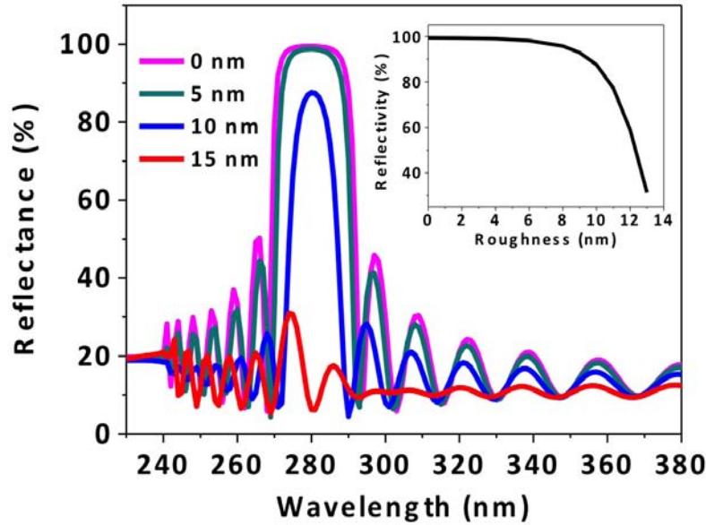
Figure 60: Simulated reflectance of 20-period B_{0.04}Al_{0.96}N (33 nm) / Al_{0.70}Ga_{0.30}N (28 nm) DBR with different values of roughness; Inset shows the curve of the central wavelength reflectivity versus the roughness.
