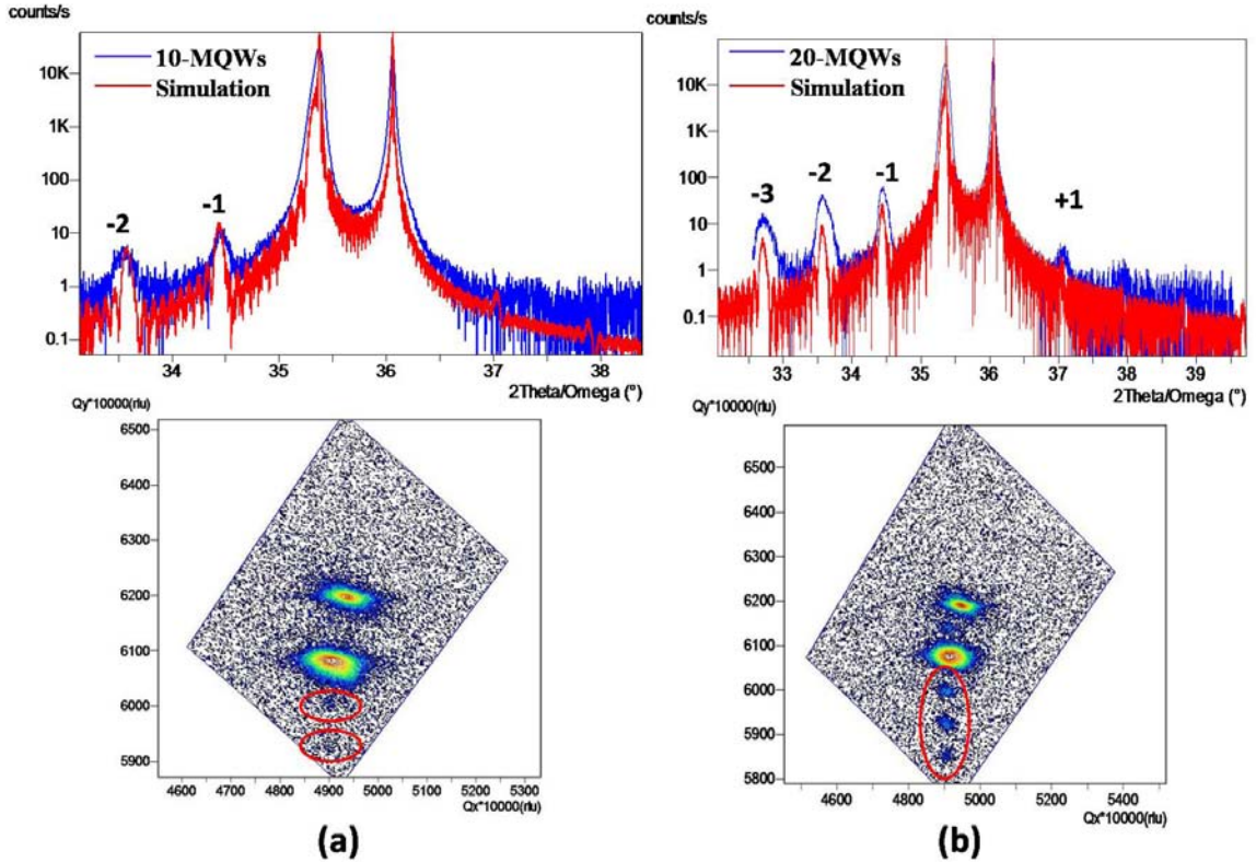
Figure 44: Symmetric 2\theta - \omega scans and (1 1 -2 4) RSMs of (a) 10-period and (b) 20-period MQWs grown on a relaxed AlGaIn buffer on AlN templates.
