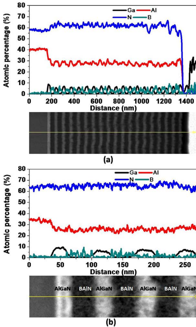
Figure 69: EDX profiles of different elements along the growth direction of 18-pair BAIN/AlGaN DBR structure reflecting at 265 nm with (a) lower and (b) higher magnification.
