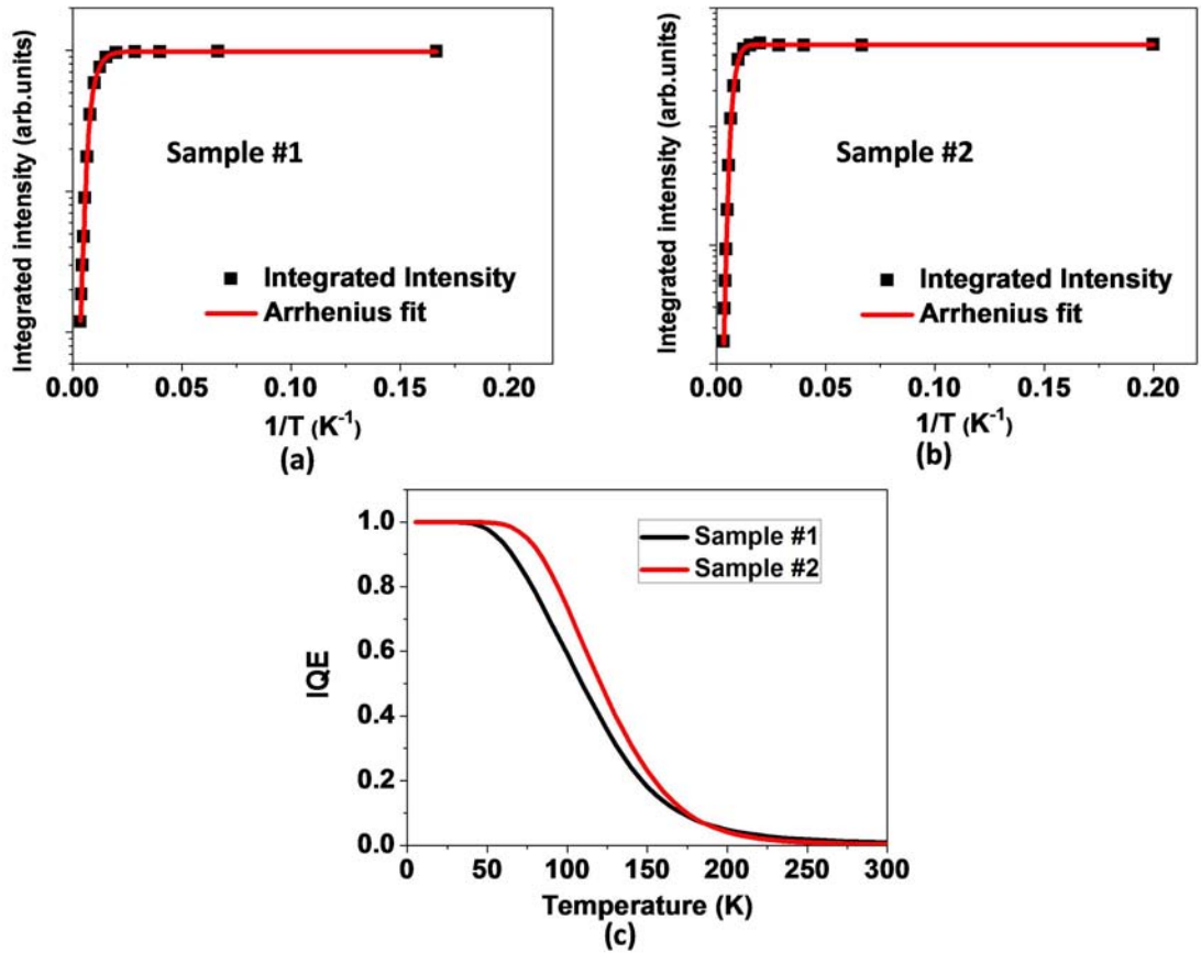
Figure 53: PL integrated intensity as function of temperature (with a cw laser and a weak excitation of \sim 1\text{W}/\text{cm}^2 ) and Arrhenius fitting for (a) sample #1 and (b) sample #2; (c) is the curve of IQE versus temperature based on Arrhenius equation fitting.
