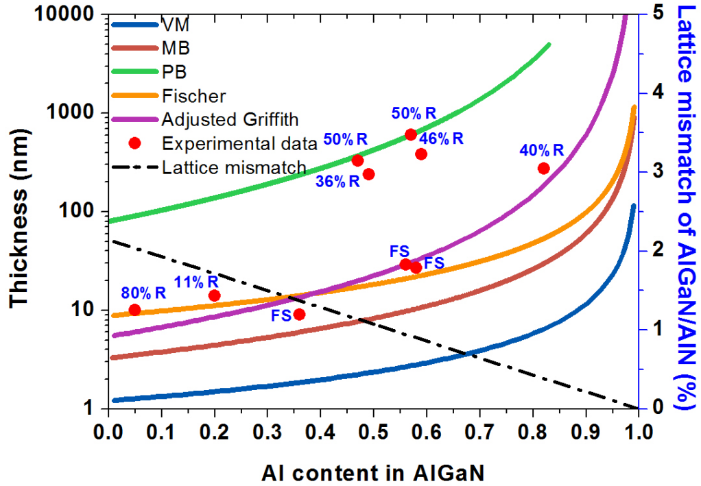
Figure 20: Critical thickness of AlGaN layers grown on AlN templates calculated by different models along with experimental data.
