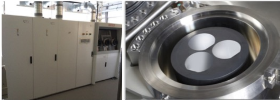
Figure 14: Aixtron 3×2 inch, close coupled showerhead (CCS) MOVPE system.
