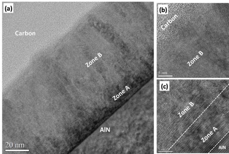
Figure 35: (a) Cross section STEM image (bright field) of 75 nm thick BAIN layers containing 12% boron along the [1\ 1\ -2\ 0] zone axis. Zone A has lattice oriented along c-axis and Zone B has columnar feature; (b) higher magnification image for the top part of the layer; (c) higher magnification image for the film/substrate interface.
