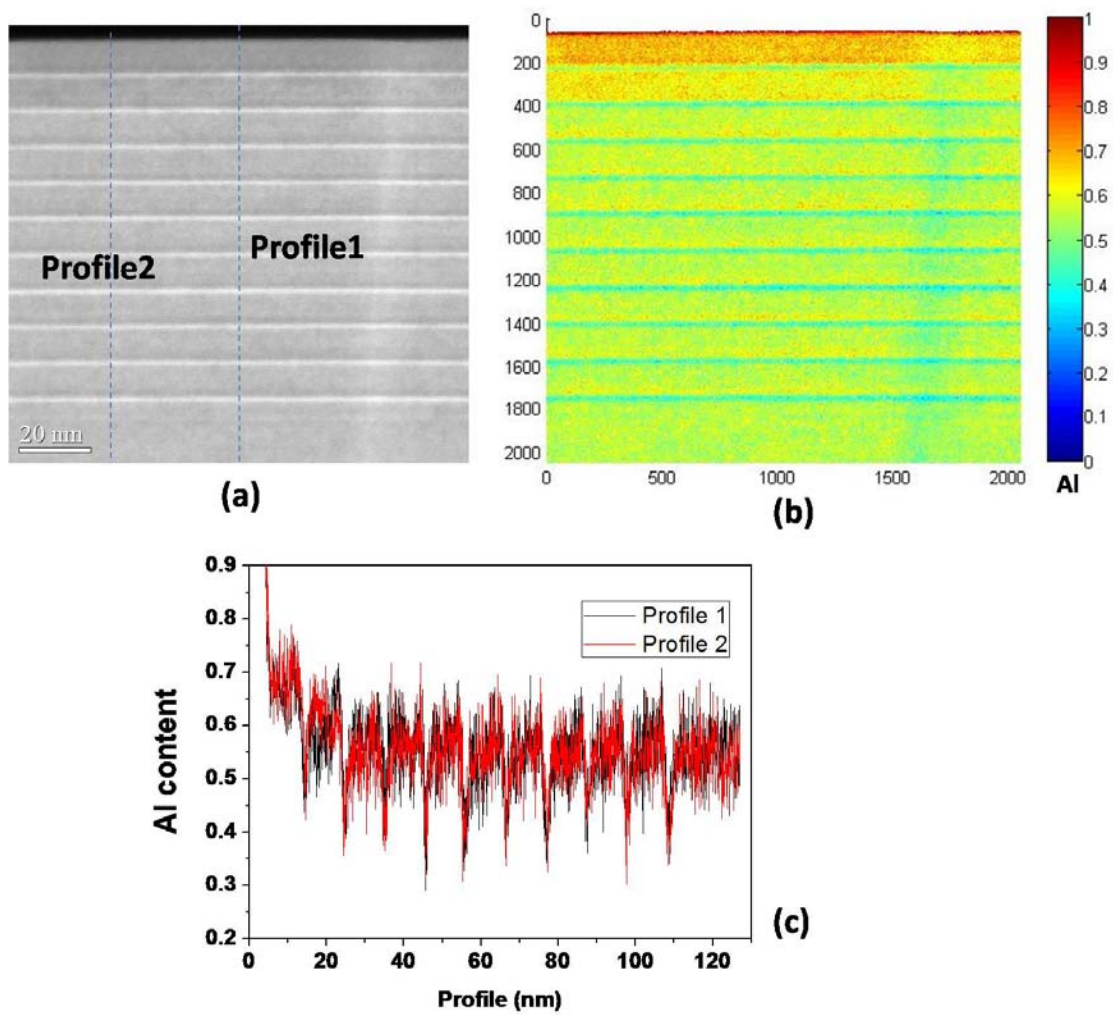
Figure 46: (a) Cross-sectional HAADF-STEM image of 10-period MQWs grown on a relaxed AlGaN buffer; (b) Compositional mapping obtained from the STEM image; (c) Al content distribution along the profiles marked in (a).
