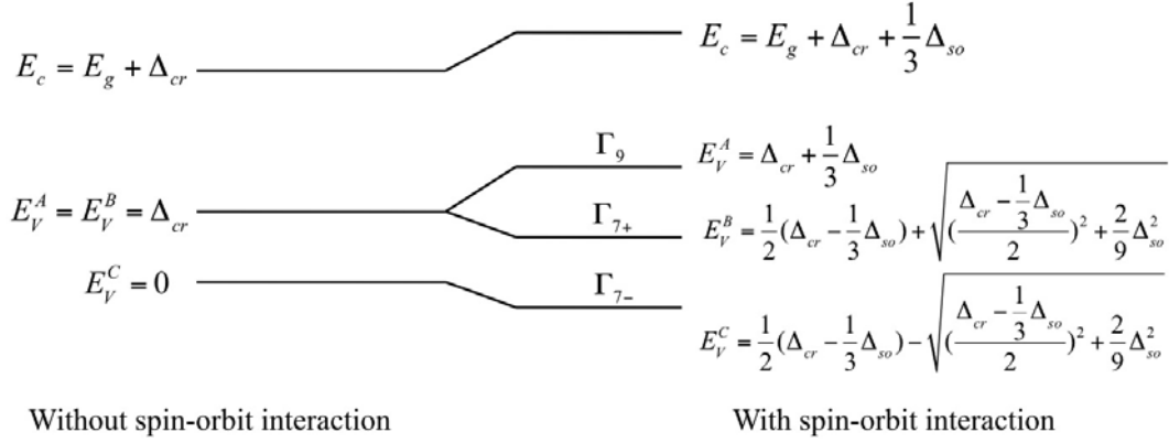
Figure 37: The band-edge energies with and without spin-orbit interaction.
