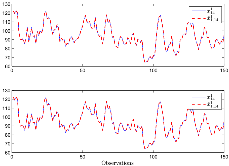
FIGURE 2.5 – Evolution des signaux x_{14}^1 , \check{x}_{1,14}^1 et \hat{x}_{1,14}^1
