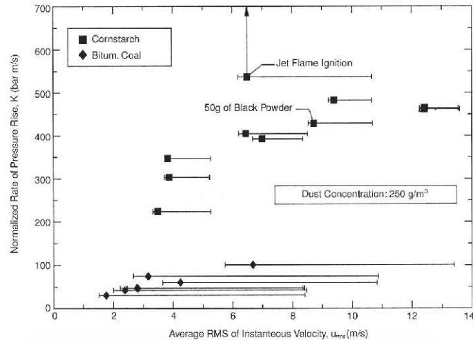
Figure 3.1. Rate of pressure rise in room-like structure as a function of RMS turbulent velocity. Data from (Tamanini, 1990), interpreted using the vent sizing correlation from (Tamanini and Valiulis, 1996)., extracted from (Tamanini, 1998)
