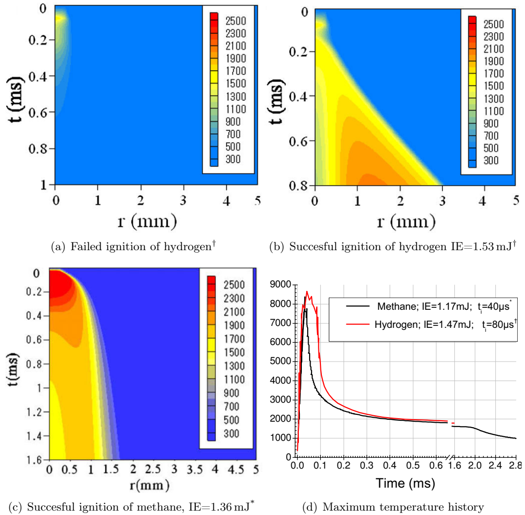
Figure 2.19. Behaviour of temperature during and after spark ignition of methane * and hydrogen † according to simulations involving detailed chemistry.
