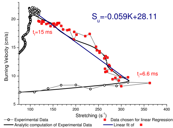
(a) Burning velocity vs stretching
