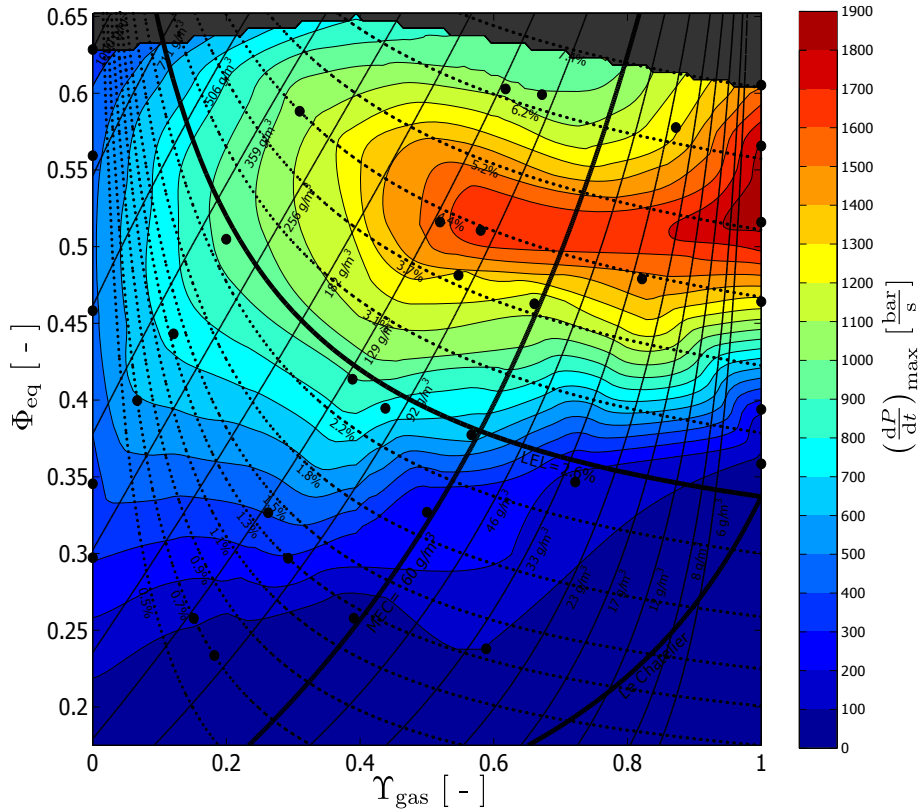
Figure 1.12. Rate of pressure rise map for the niacin/acetone mixtures with t_v = 60 ms. \Upsilon_{\text{gas}} and \Phi_{\text{eq}} are defined by Equations 1.25 and 1.28 respectively. y_{\text{gas}} and C_{\text{dust}} are represented by the pointed and solid lines respectively. (Sanchirico et al., 2011)
