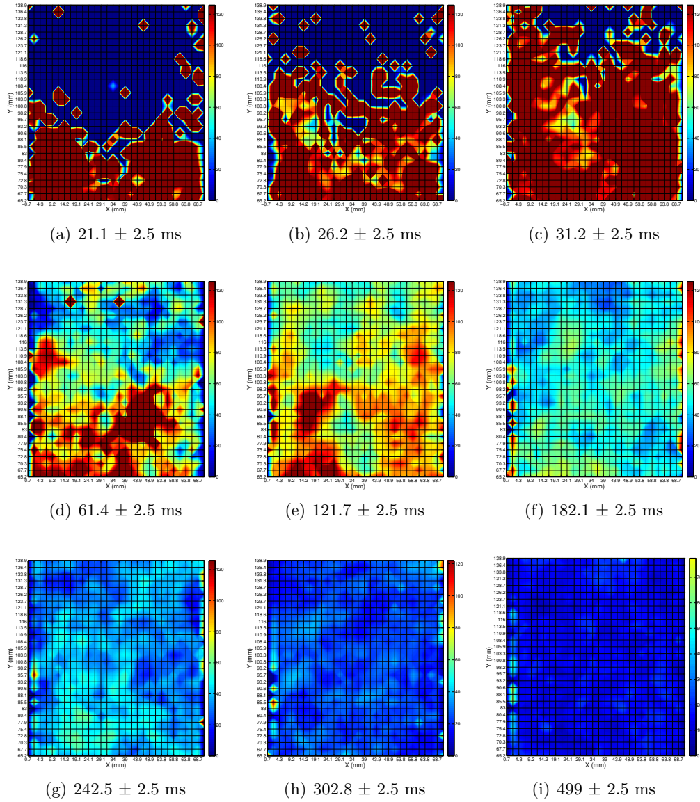
Figure 3.11. Turbulence intensity map for different times
