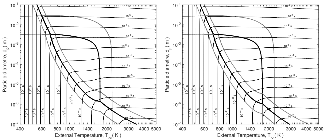
(e) Process times with Di Blasi and Branca (2001) kinetics (f) Process times with Wagenaar et al. (1993) kinetics
