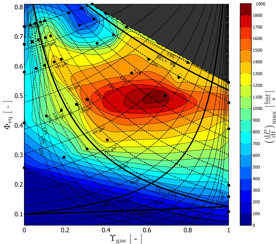
Figure 1.14. Rate of pressure rise map for the telithromycine/toluene mixtures. \Upsilon_{\text{gas}} and \Phi_{\text{eq}} are defined by Equations 1.25 and 1.28 respectively. y_{\text{gas}} and C_{\text{dust}} are represented by the pointed and solid lines respectively. (Dufaud et al., 2009)
