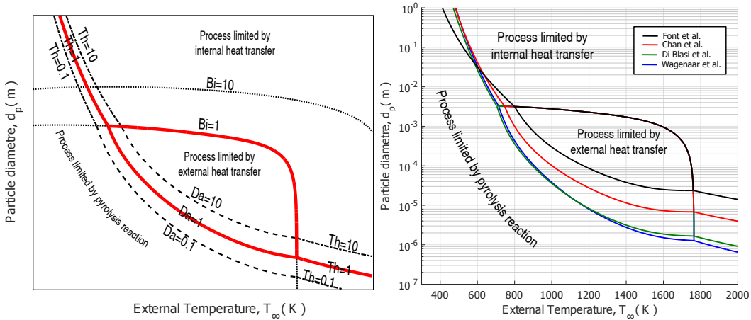
(a) Description of the construction of the limits for each regime (b) Consolidated regime limits for each kinetic model
