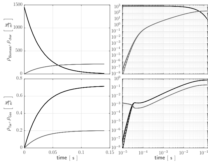
(b) Densities
