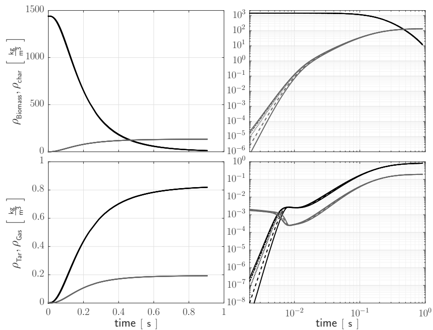
(b) Densities
