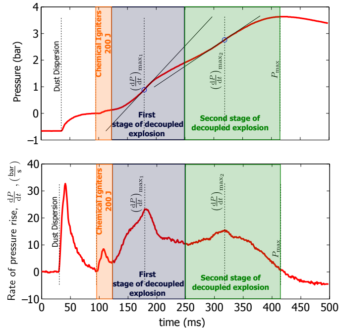
Figure 1.19. Decoupled explosion in sinergic regime. Explosion produced in the 20L with a hybrid mixture of starch at 106.6 \frac{\text{g}}{\text{m}^3} and methane at 3.41 %vol, t_v = 60 ms and chemical igniters of 200 J.
