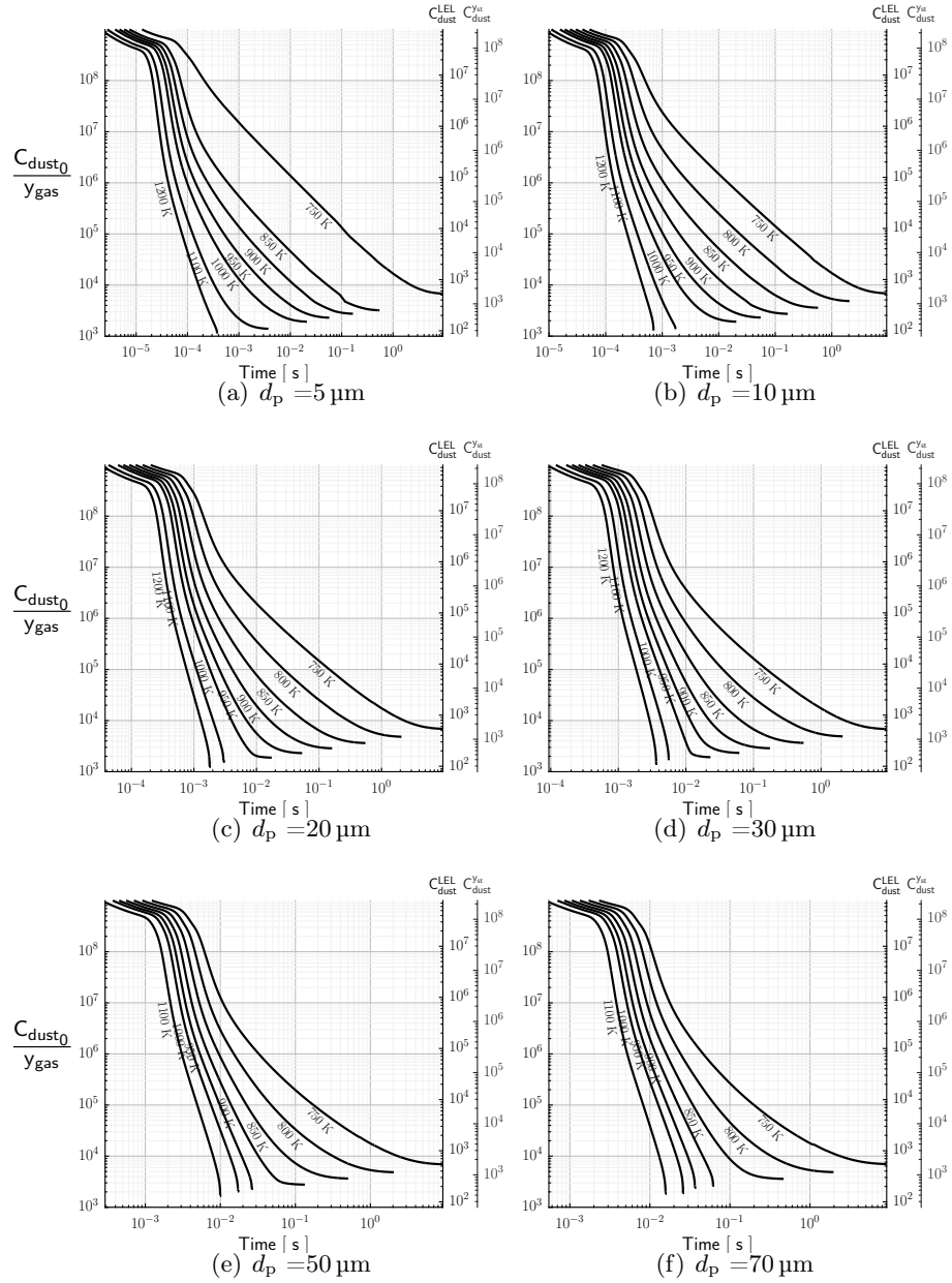
Figure C.9. Initial C_{\text{dust}} necessary to reach a concentration of y_4 in pyrolysis gases at time t using Wagenaar kinetics, auxiliary axes on the left show the initial concentration necessary to reach the LEL = 7.8% and the stoichiometric concentration (23%) of pyrolysis gases. Units for C_{\text{dust}} are in \frac{\text{g}}{\text{m}^3} .
