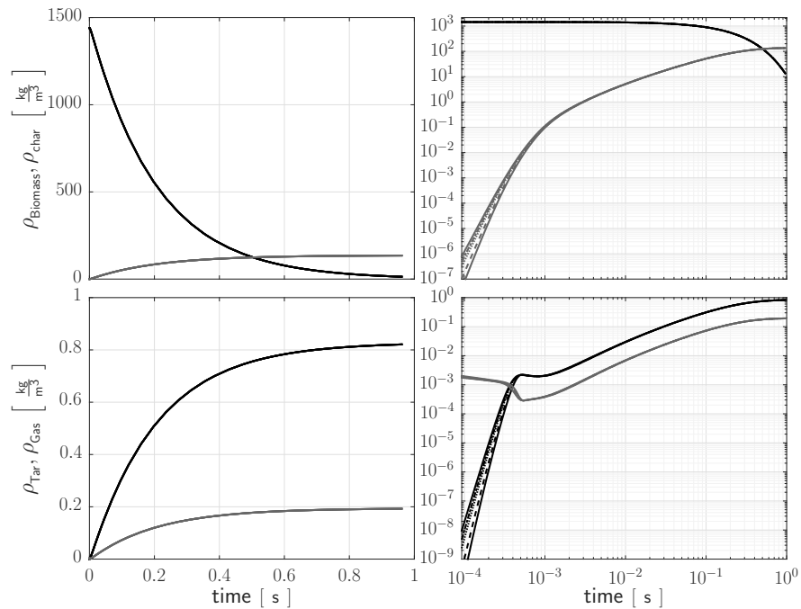
(b) Densities
