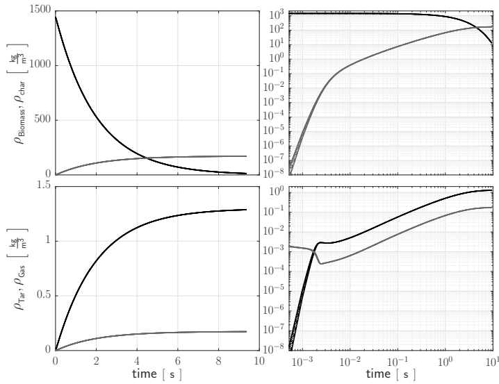
(b) Densities
