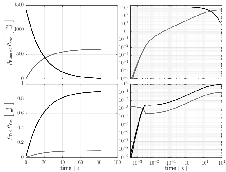
(b) Densities
