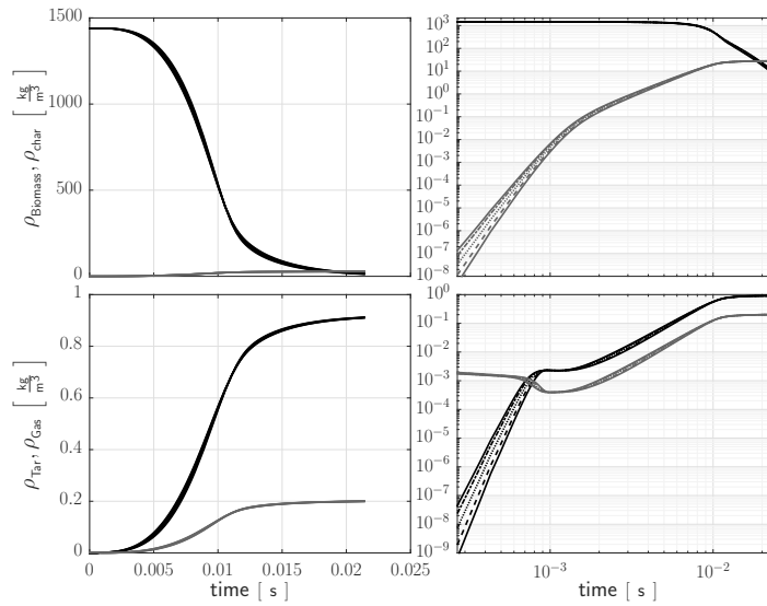
(b) Densities
