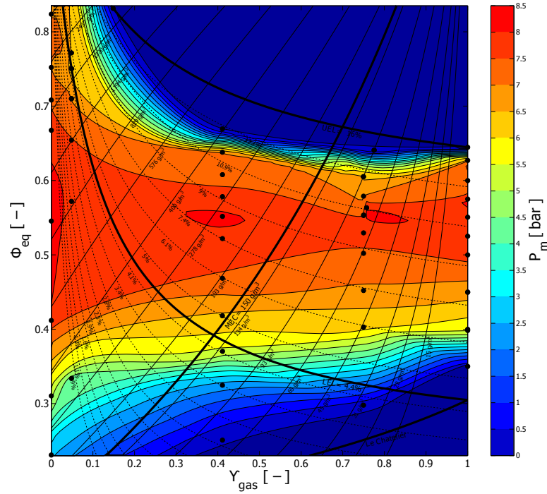
Figure 1.18. Overpressure map for the starch/methane mixtures. \Upsilon_{\text{gas}} and \Phi_{\text{eq}} are defined by Equations 1.25 and 1.28 respectively. y_{\text{gas}} and C_{\text{dust}} are represented by the pointed and solid lines respectively
