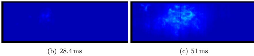
Figure 4.12. Estimation of characteristic flame parameters of methane and starch, 1.92% (v/v) and 1048 mg respectively, t_v = 120 ms
