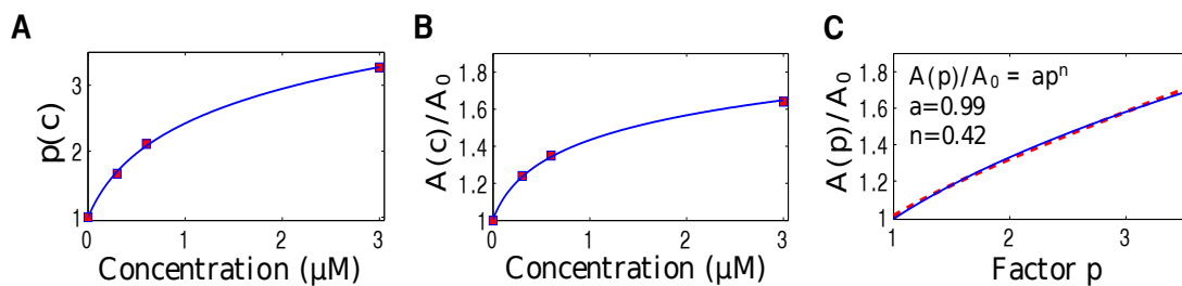
Fig. 3.1. Effect of propofol on thalamic \text{GABA}_A -receptors extracted from a previous experimental study [79, Fig. 5]. (A) The factor p = \beta_i^0/\beta_i of evoked IPSCs in a relay neuron (taken from the experimentally measured normalized decay time) subject to the propofol on-site concentration c (red square) and the corresponding fitted function (blue line) p(c) = k_1 \ln(k_2 + k_3c) . (B) The experimentally measured normalized amplitude A(c)/A_0 of evoked IPSCs subject to the propofol on-site concentration c (red square) and the corresponding fitted function (blue line) A(c)/A_0 = k_4 \ln(k_5 + k_6c) . Here A_0 = A(c = 0) . (C) Since the constants k_1, \dots, k_6 are fitted, A_r(p) = A(p)/A_0 = k_4 \ln(k_7 + k_8 \exp(p/k_1)) (red line) with k_7 = k_5 - (k_2k_6/k_3) , and k_8 = k_6/k_3 . An additional fit reveals A(p)/A_0 \approx p^{0.42} (blue line).
