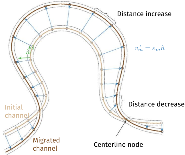
Figure 4.4 Migration principle: the centerline nodes are moved along a migration vector \vec{v}_m based on the normal \hat{n} to the centerline and a migration factor \epsilon_m . \hat{s} is the normalized vector along the streamwise direction.
