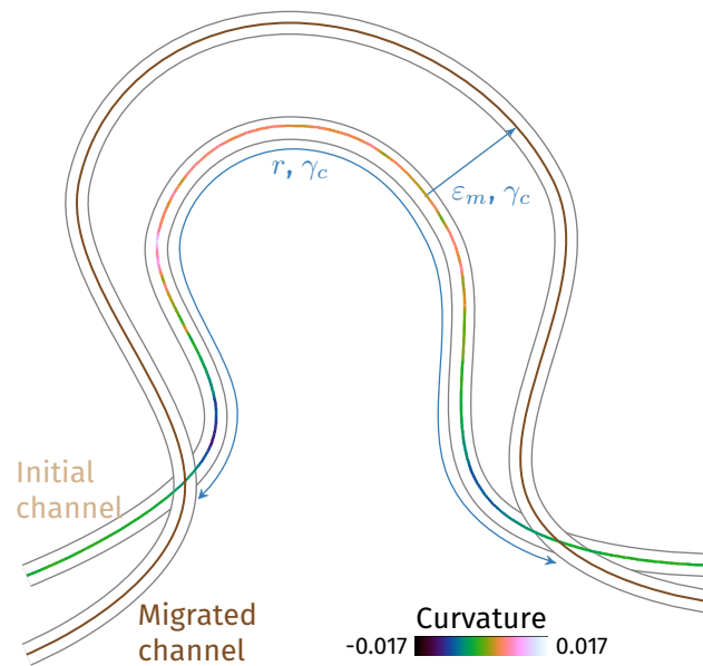
Figure 4.6 Main parameters used for horizontal bend migration with SGS. \varepsilon_m is the migration factor, r the variogram range and \gamma_c the curvature weight. The later perturbs the two other parameters by fitting more or less the migration spatial structure to the curvature spatial structure.
