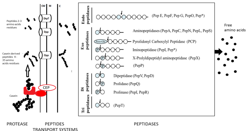
Figure 7 : Proteolysis pathway by LAB, adapted from Doeven (Doeven et al., 2005), Christensen (Christensen et al., 1999) and Savijoki (Savijoki et al., 2006) with schematic representation of the action of peptidases found in lactic acid bacteria. Amino acids are symbolized by a circle and the arrow indicates the cleavage site. P: proline; *, unclassified Endopeptidases.
