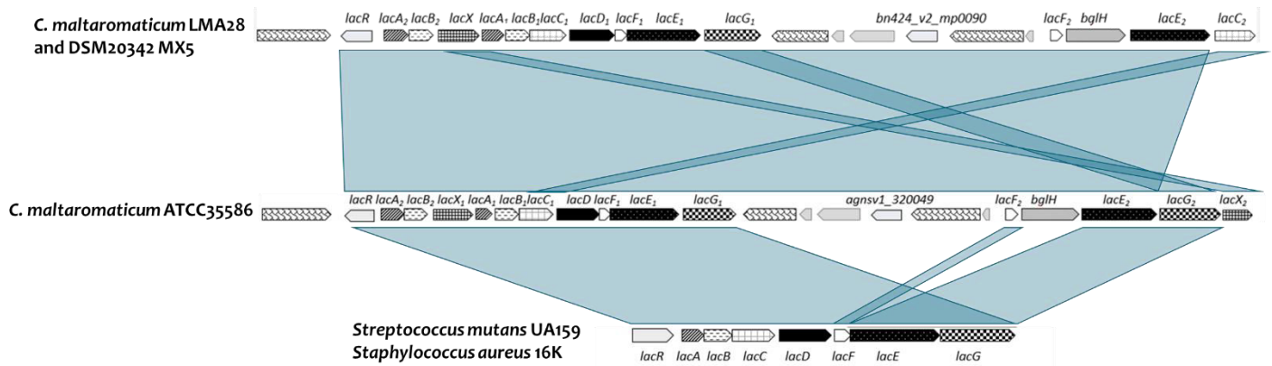
Figure 16: Organization and synteny between lac genes among Carnobacterium maltaromaticum LMA28, DSM20342-MX5, ATCC35586, Streptococcus mutans , and Staphylococcus aureus .
