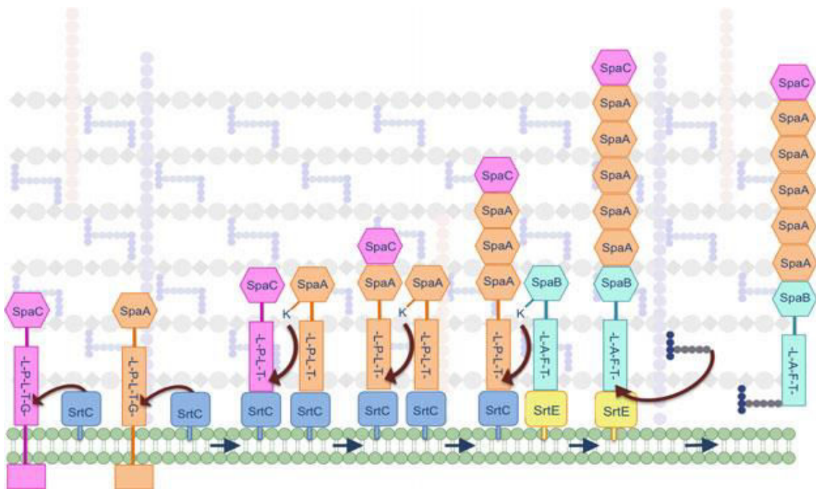
Figure 6 : Model of pilus biogenesis (Bradshaw et al., 2015). SpaA backbone pilin, SpaC tip pilin, SpaB base pilin, srtA sortase A, srtC sortase C, srtE sortase E, LPLTG and LAFT anchorage domains of pillins.
