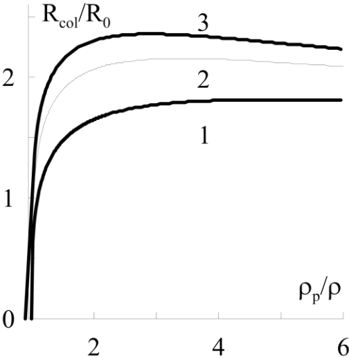
Fig. 4.5. Dependence of particle collision radius with a bubble with radius of 500 mkm on particle density in acoustic field with \omega = 40000 rad/s frequency and 1500 Pa acoustic pressure. Radius of particle is 100 mkm (3), 70 mkm (2), 40 mkm (1)
