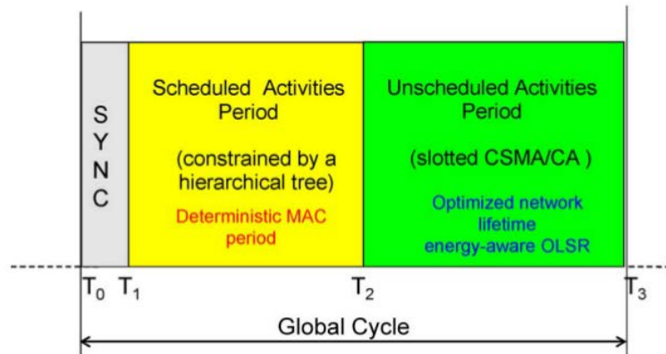
FIGURE 3.26 – Structure d'un cycle du protocole MaCARI. (Source : [Agha et al., 2009] figure 3)
