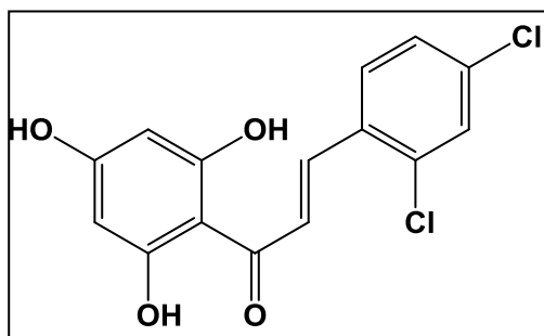
Figure 41: 2,4-dichloro-2',4',6'-trihydroxychalcone
