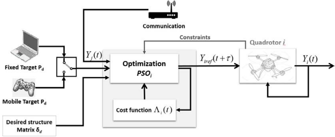
FIGURE 3.3 – General scheme
