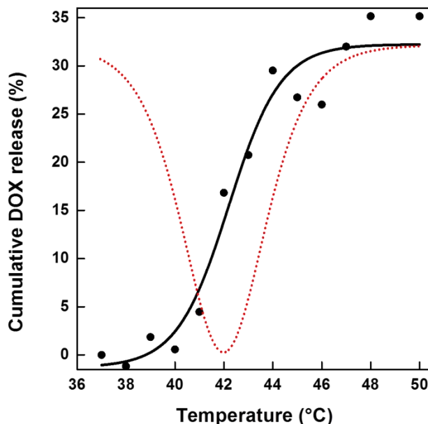
Figure 4.3.14 Cumulative DOX release profile of \text{Fe}_3\text{O}_4@P(\text{MEO}_2\text{MA}_{60}\text{-OEGMA}_{40})\text{-DOX} dispersed in CM.
