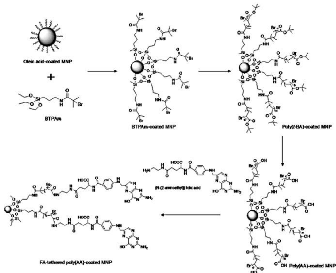
Figure 1.2.4 Surface modification of \text{Fe}_3\text{O}_4 with poly(AA) [210].
