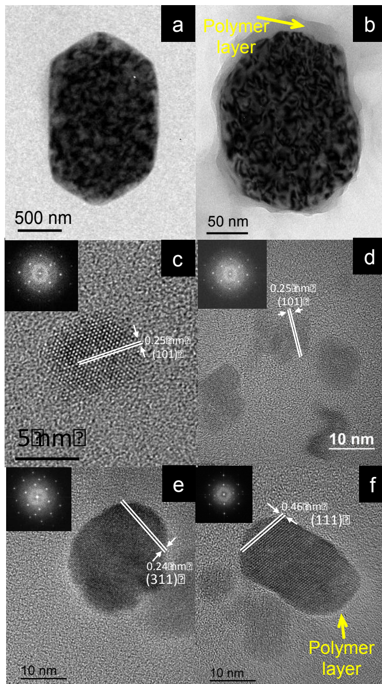
Figure 2.3.2 HR-TEM micrographs of a) SiO 2 @Ph-Cl NPs, b) SiO 2 @PS after 8 h of polymerization, c) ZnO@Ph-Cl NPs, d) ZnO@P(MEO 2 MA 80 -OEGMA 40 ) NPs, e) Fe 3 O 4 @Ph-Cl NPs, and f) Fe 3 O 4 @P(MEO 2 MA 80 -OEGMA 40 ) NPs (the insets of figures 2c-f correspond to the FFT).
