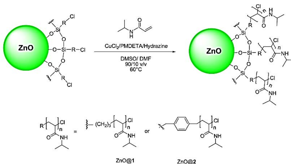
Figure 1.1.48 Schematic representation of the surface-initiated ARGET-ATRP polymerization of NIPAM from \text{ZnO@1} and \text{ZnO@2} NPs.
