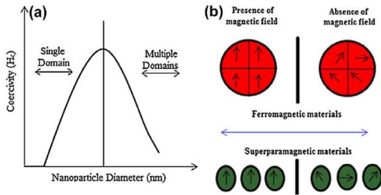
Figure 1.1.20 Relationship between magnetization behavior of NPs size and the magnetic domain structures.
