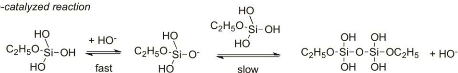
Figure 13: Hydrolysis and condensation of TEOS catalyzed by acid or base.
