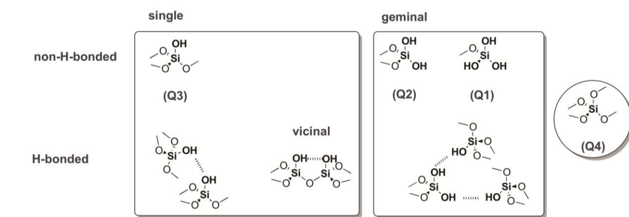
Figure 12: Types of silanol and silica bridges.
