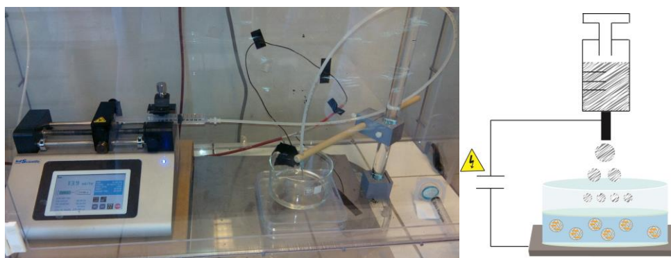
Figure 17: (left) Electrospraying setup used for the obtainment of the alginate beads, (right) alginate beads formation cartoon.
