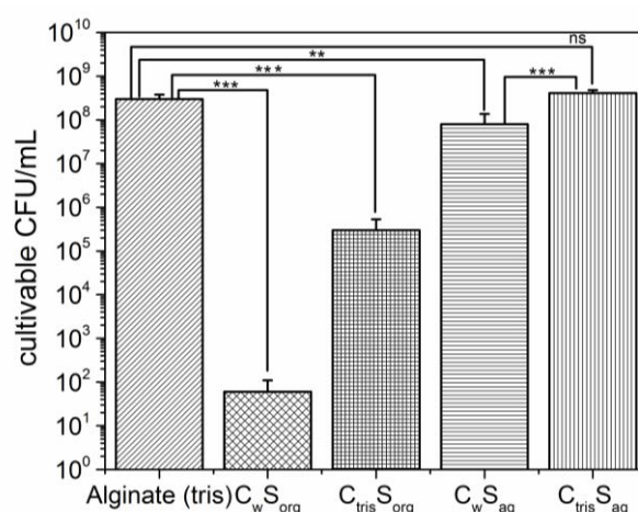
Figure 48: LGG viability studies in different synthesis conditions. The results are expressed as the average of three independent experiments. Error bars indicate standard deviations. Error bars indicate standard deviations. Comparisons were done between all pairs of columns. ** p < 0.01 , *** p < 0.001 and ns stands for not significant difference.
