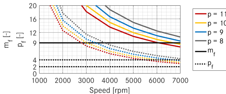
Figure 68: Frequency modulation ratio ( m_f ) and pulse number per half-cycle ( p_f ) variations
