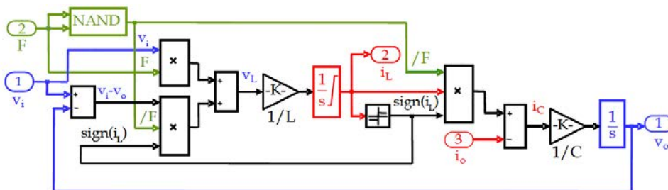
Figure 63: Boost-converter modeling from [82]
