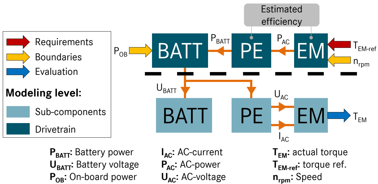
Figure 121: Present approach for the design of electric drive system for hybrid electrical drivetrains
