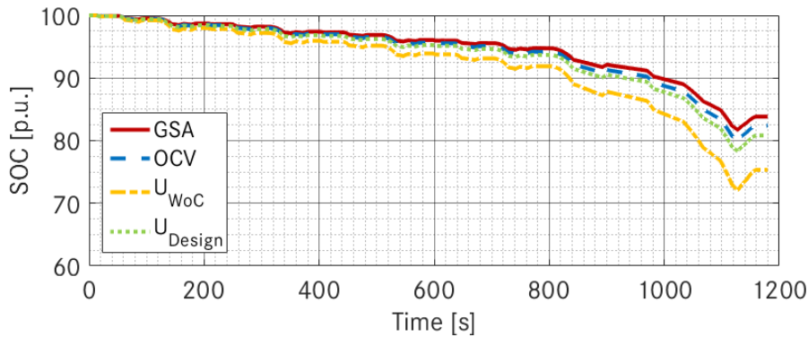
Figure 154: State of charge over time for the different methods
