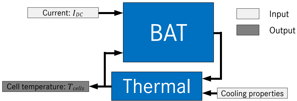
Figure 111: Modeling approach for the validation of the thermal modeling
