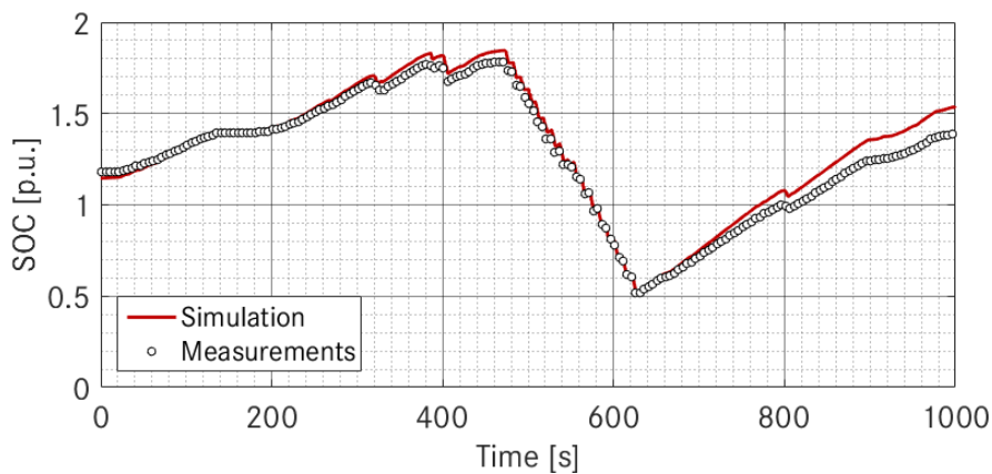
Figure 141: SOC comparison with vehicle measurements
