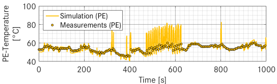
Figure 144: PE-temperature comparison with measurements
