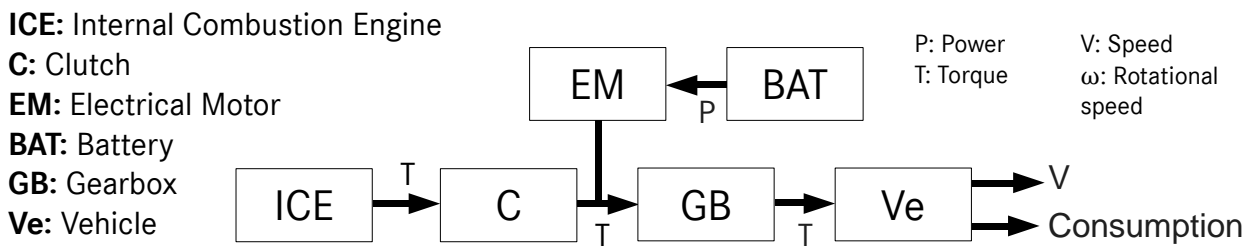
Figure 20: Representation of a hybrid electrical vehicle with the forward approach based on [61] and [62]
