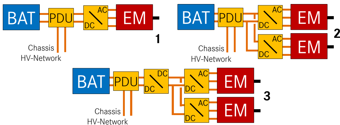
Figure 10: Electrical architectures in hybrid electrical drivetrains [23], [24] and [34]
