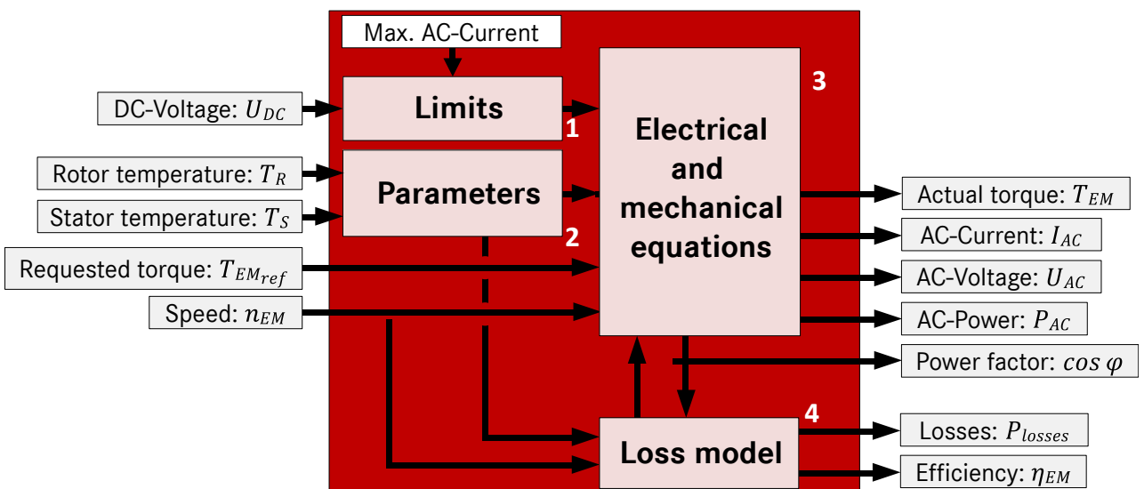
Figure 34: Circuit based modeling approach
