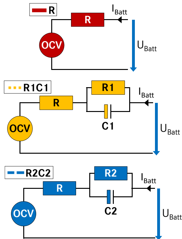
Figure 105: Investigated circuit for the battery modeling comparison
