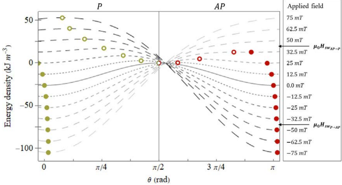
Figure II.9: Energy density of a magnetic tunnel junction with a tilted applied field direction ( 5^\circ from the z -axis) as a function of the polar angle \theta for applied magnetic fields from 75mT (light gray) to -75 mT (dark gray), by steps of 12.5mT. The full green (red) dots represent the P(AP) state as a minimum of energy density, the empty dots represent the corresponding state as a maximum of energy density.
