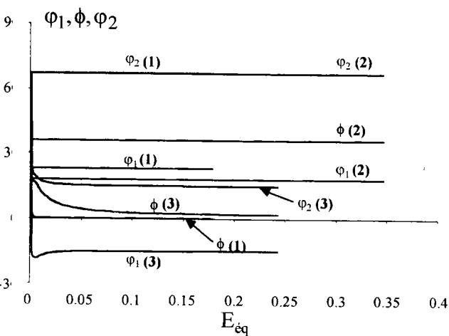
Figure III.9e: angles d'Euler
