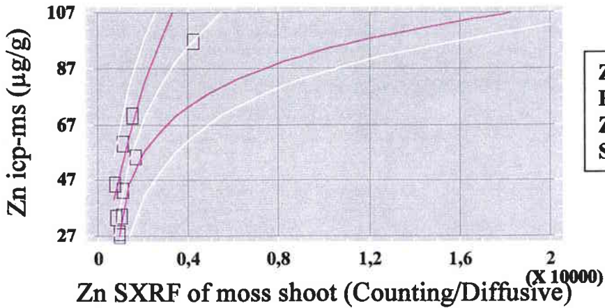
FIGURE 3 : Examples of linear and logarithmic regression models between ICP-MS ( \mu\text{g/g} ) (dependant variables) and in vivo SXRF (counting/diffusive ratio) (independant variables) data for Pb and Zn. R^2 indicates the % of the variability explained by the model and S_r is the standard error of estimation. The equation of the model is shown as the white inner solid line. The plots include both confidence limits for the means (inner pink lines) and prediction limits (outer dotted white lines).
