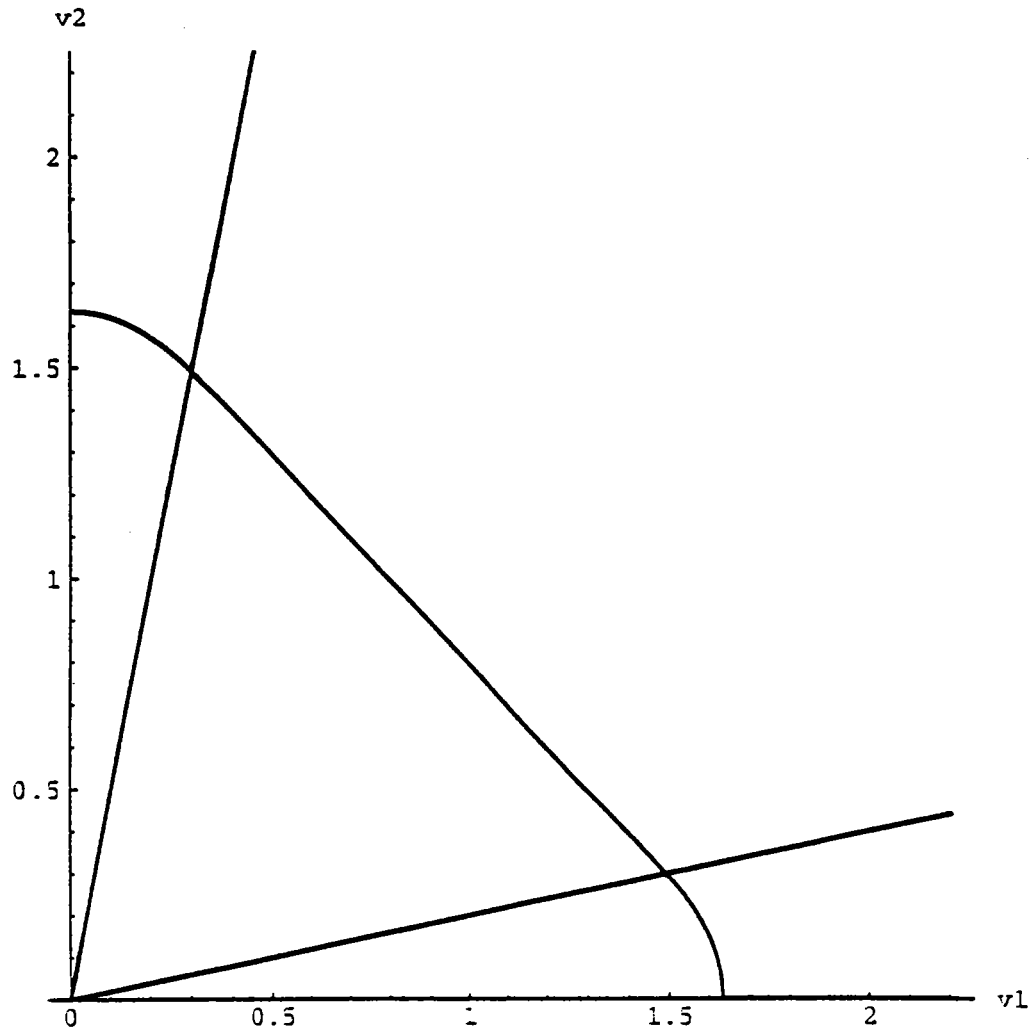
Figure 2 : \frac{\lambda}{\mu} = 3
