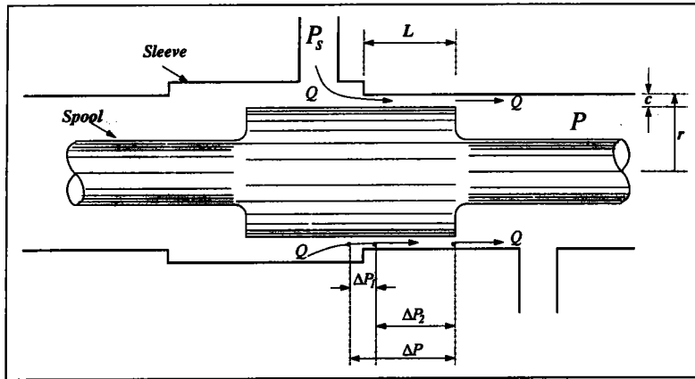
FIG. 2.13 – A spool valve at an overlapped position
