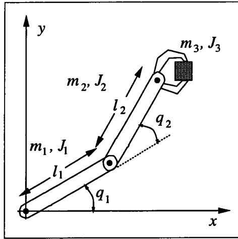
FIG. 6.1 – Two-link planar robot arm
