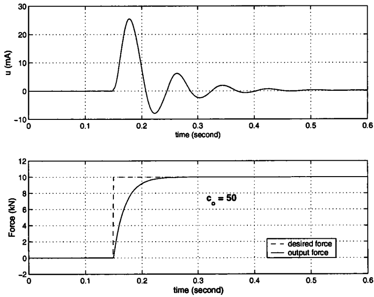
FIG. 3.2 – Force behaviour and needed control law. (tracking constant force)
