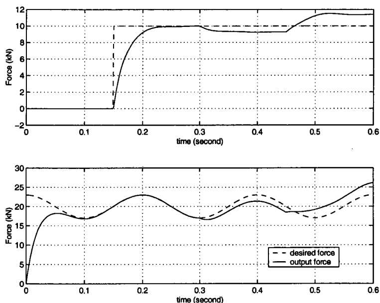
FIG. 3.5 – State behaviour of the system with linearizing feedback control, undergoing parameter uncertainties.
