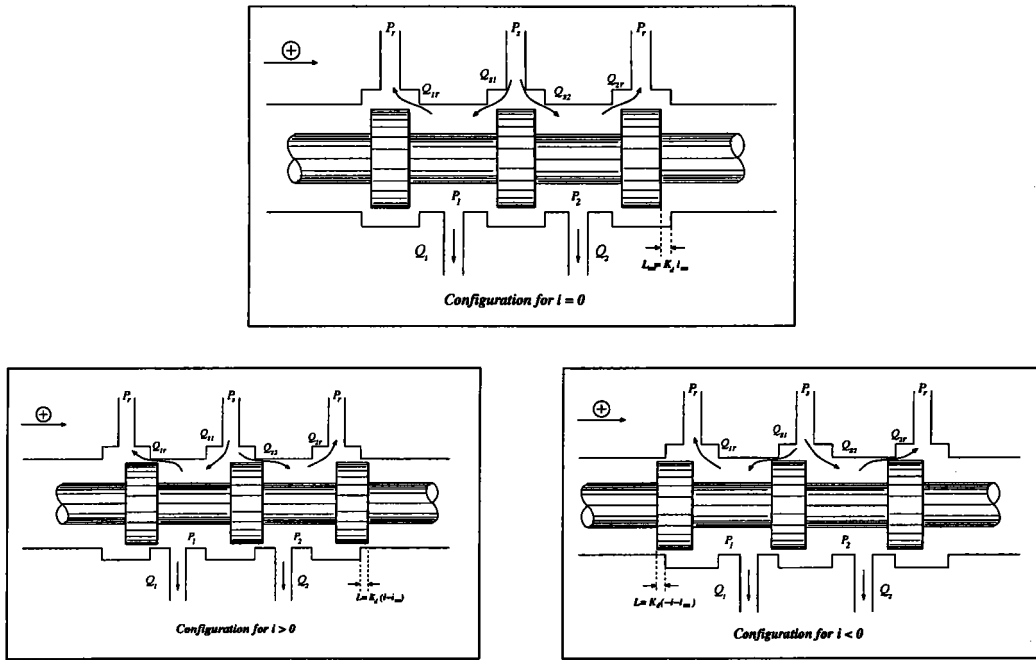
FIG. 2.20 – Underlapped spool valve in different positions
