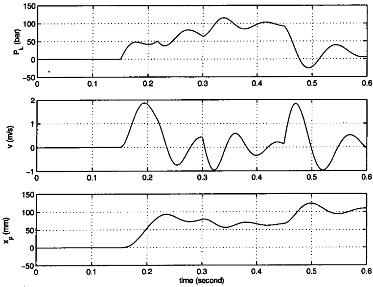
FIG. 3.6 – State behaviour of the system. (tracking constant force)
