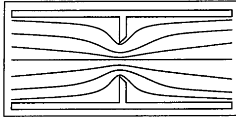
FIG. 2.12 – Laminar flow through a sharp-edged orifice
