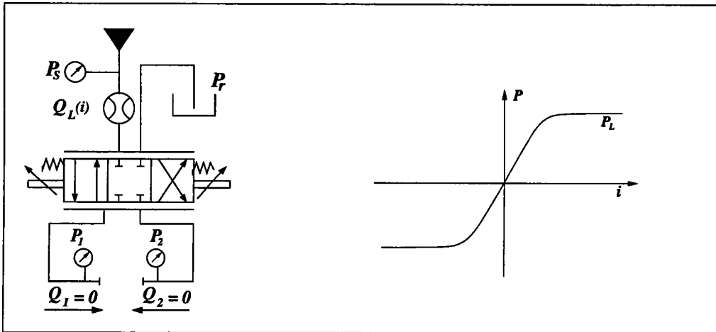
FIG. 2.8 – Block-line pressure sensitivity curve
