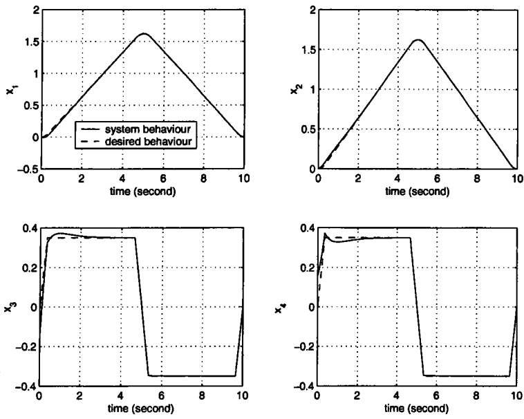
FIG. 6.3 – Output tracking using state feedback.
