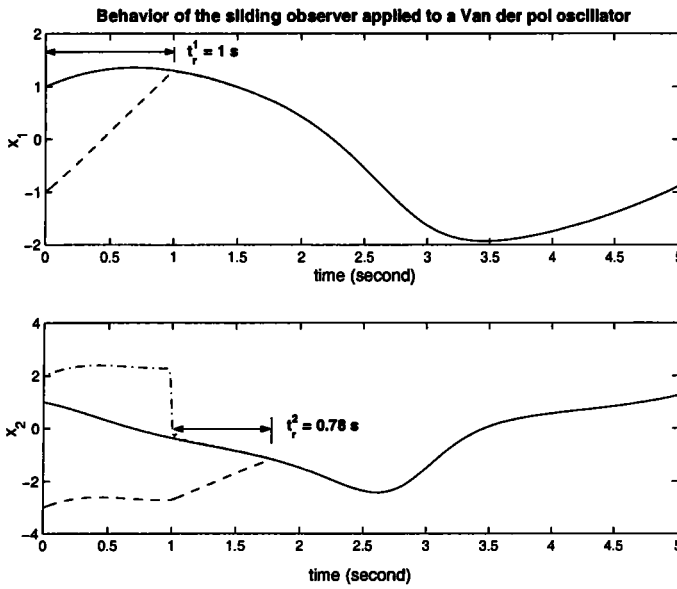
FIG. 4.4 - x (—), \hat{x} (- - -), \xi (- · - · -) x_1(0) = 1, x_2(0) = 1 , \hat{x}_1(0) = -1, \hat{x}_2(0) = -3 w_1 = 5 and w_2 = 3
