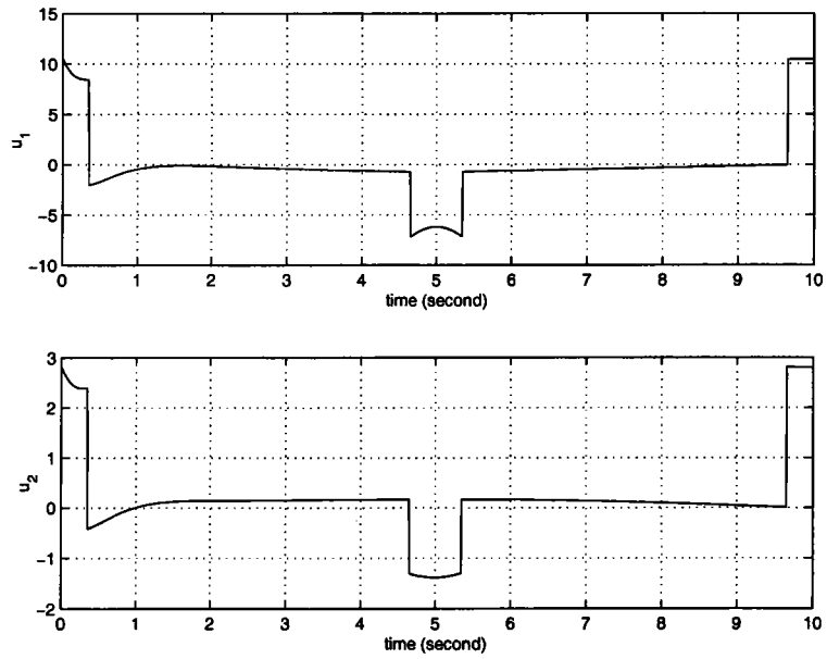
FIG. 6.7 – Feedback control constructed using observer states.
