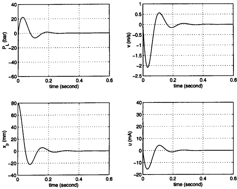
FIG. 3.11 – State behaviour and needed control law.
