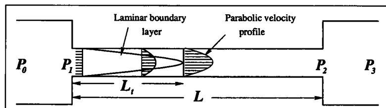
FIG. 2.9 – Laminar flow in a pipe
