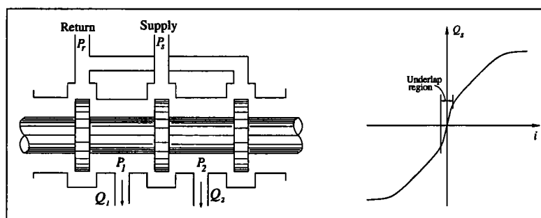
FIG. 2.3 – Open center spool valve
