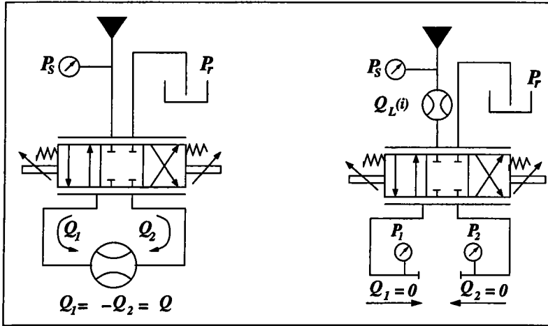
FIG. 2.17 – Setups for characteristics tests.
