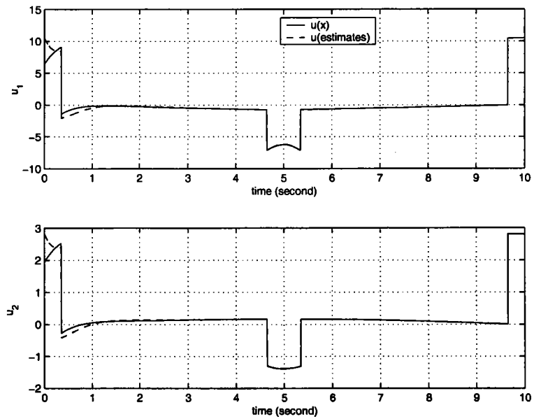
FIG. 6.8 – Comparing u(x) and u(\hat{x})
