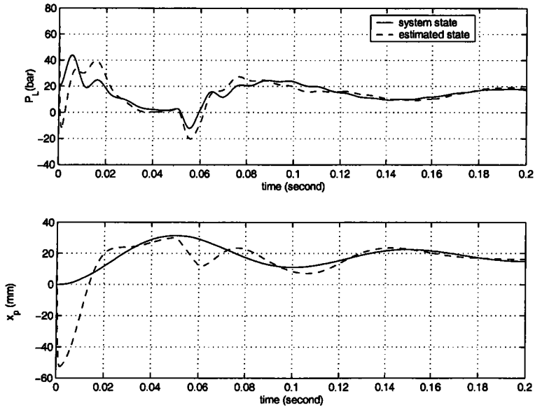
FIG. 5.5 – The high-gain observer states response to dry friction perturbation.
