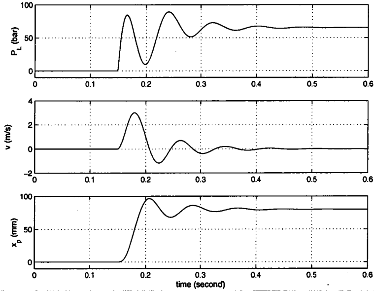
FIG. 3.1 – State behaviour of the system. (tracking constant force)
