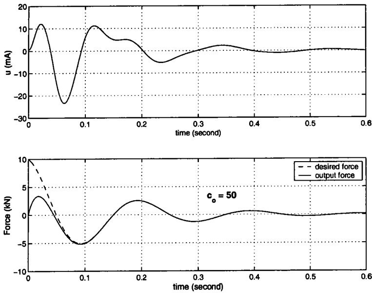
FIG. 3.4 – Force behaviour and needed control law. (tracking time-varying force)
