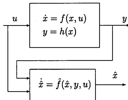
FIG. 1.3 – System observer
