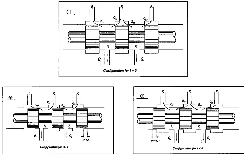
FIG. 2.16 – Critically lapped spool valve in different positions
