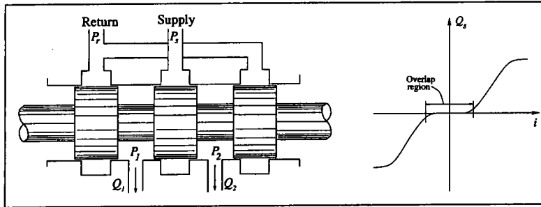
FIG. 2.4 – Closed center spool valve
