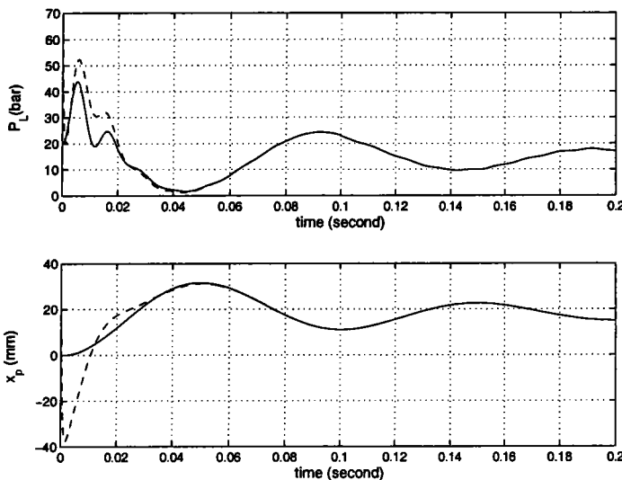
FIG. 5.4 – The high-gain observer states behaviour under no unknown inputs.
