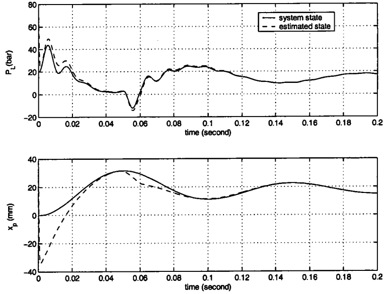
FIG. 5.7 – The sliding observer states robustness to dry friction perturbation.
