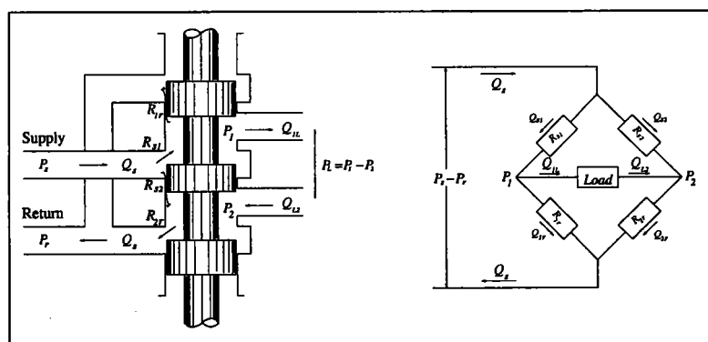
FIG. 2.1 – Wheatstone bridge
