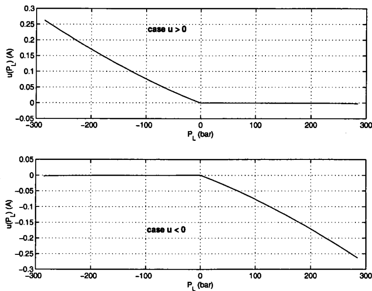
FIG. 3.10 – u(x) versus x_1 .
