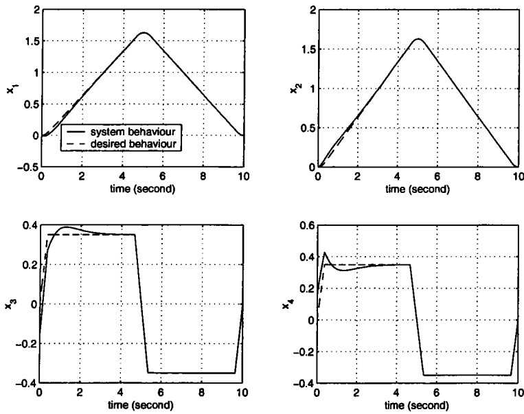
FIG. 6.6 – Tracking via observer states feedback.
