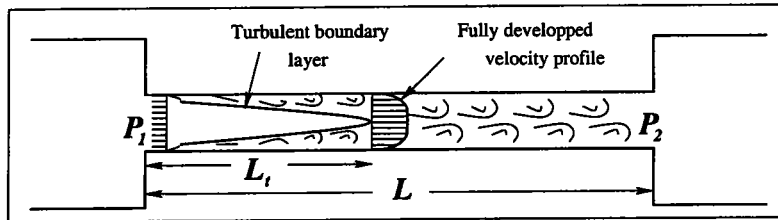
FIG. 2.10 – Turbulent flow in a pipe
