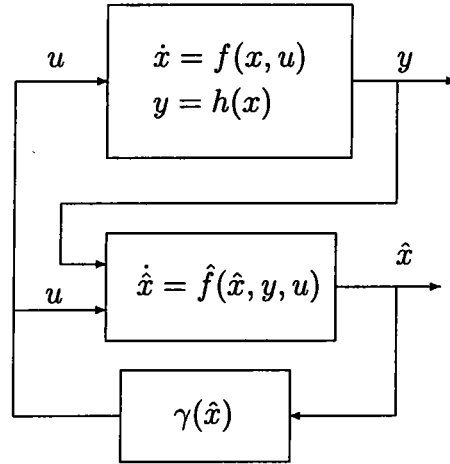
FIG. 1.4 – Controller using estimated states
