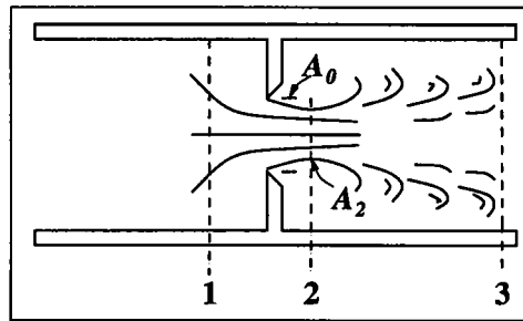
FIG. 2.11 – Turbulent flow through a sharp-edged orifice
