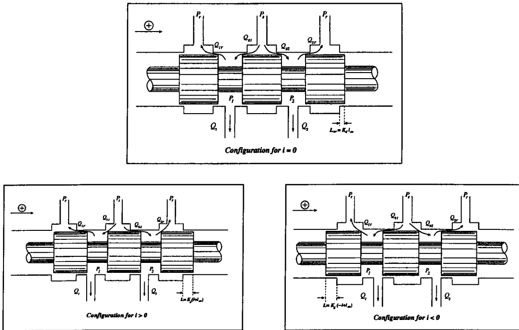
FIG. 2.21 – Overlapped spool valve in different positions
