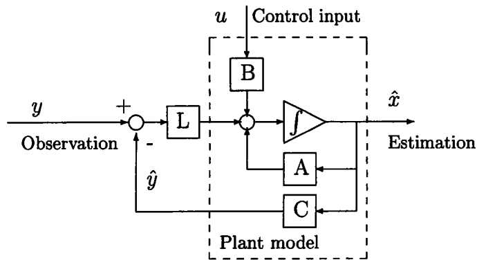
FIG. 4.2 – Full-order observer for linear systems
