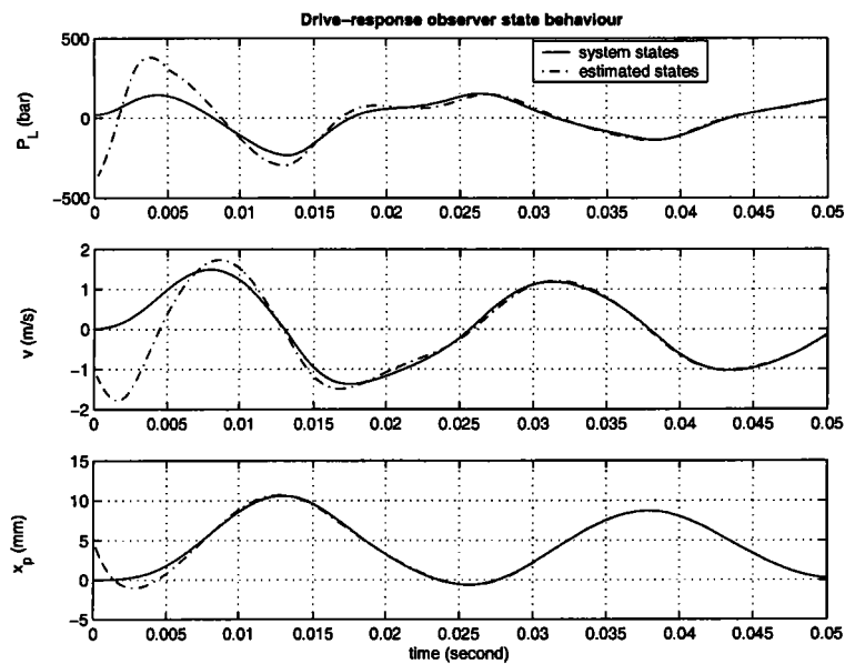
FIG. 5.3 – The drive-response observer states behaviour.
