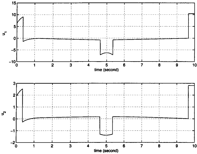
FIG. 6.4 – The needed control constructed using state feedback.
