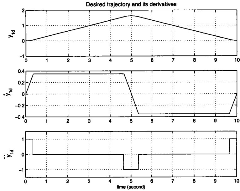
FIG. 6.2 – The desired trajectory.
