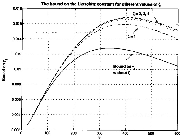
FIG. 5.1 – The upper bound on the Lipschitz constant with different design parameters.
