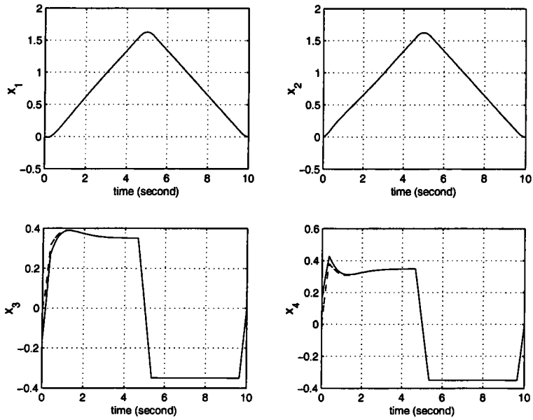
FIG. 6.5 – The observer behaviour, x(-) , \hat{x}(- -) .
