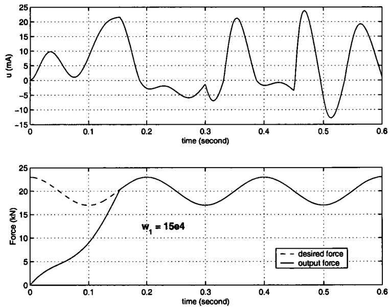
FIG. 3.9 – Force behaviour and needed control law. (tracking time-varying force)
