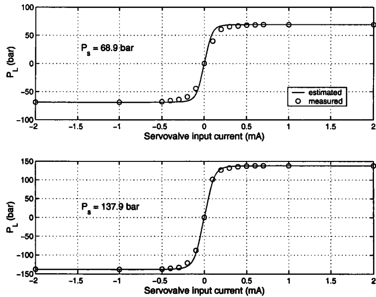
FIG. 2.19 – Measured and estimated pressure sensitivity
