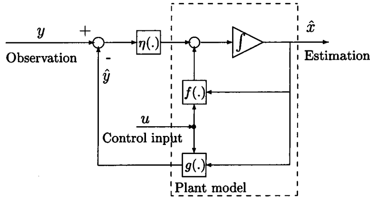
FIG. 4.3 – Structure of nonlinear observer.
