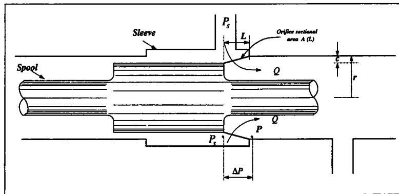
FIG. 2.14 – A spool valve at an underlapped position
