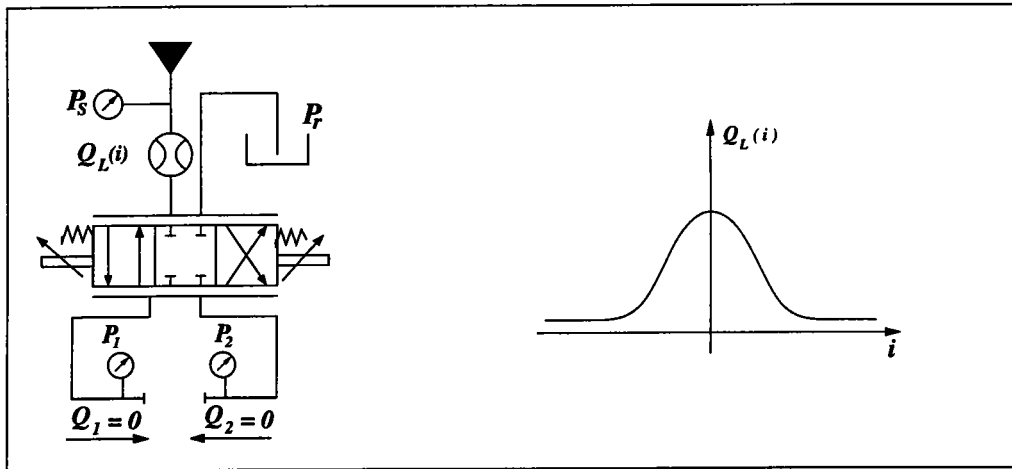
FIG. 2.7 – Setup to measure the internal leakage flow
