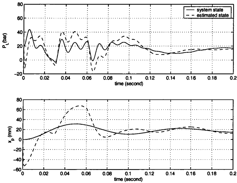
FIG. 5.6 – The high-gain observer states response to stiffness variations.
