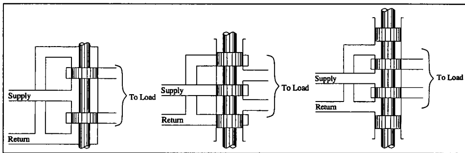
FIG. 2.2 – Typical hydraulic servovalves
