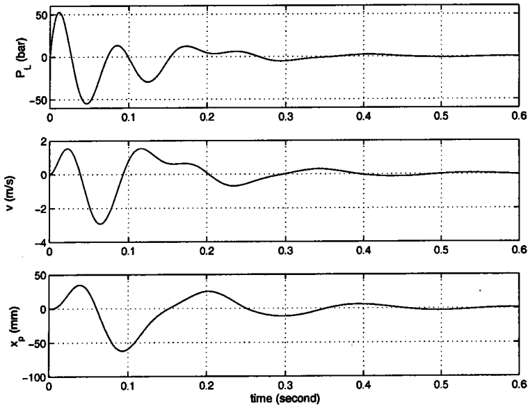
FIG. 3.3 – State behaviour of the system. (tracking time-varying force)
