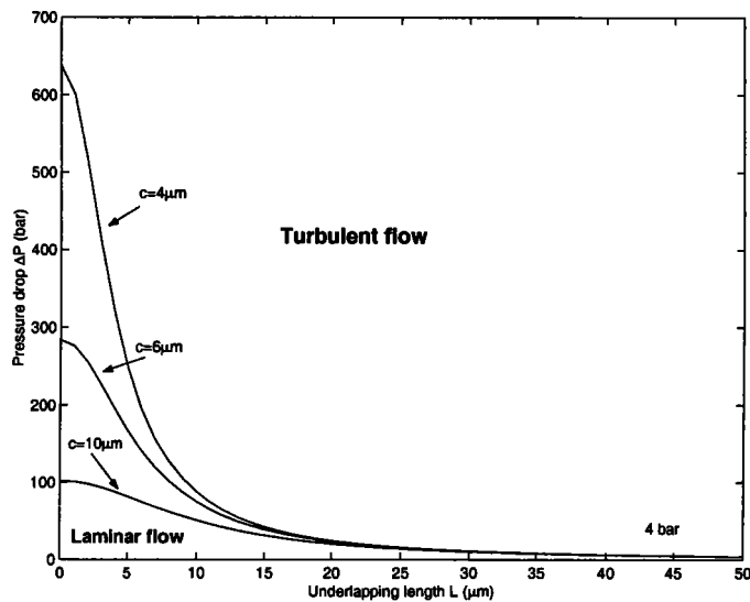
FIG. 2.15 – Laminar-turbulence transition curves
