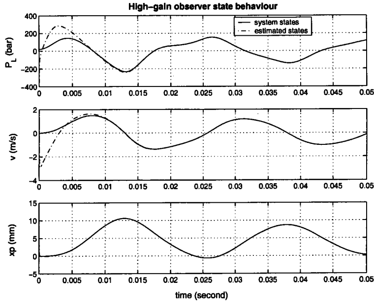
FIG. 5.2 – The observer states behaviour.
