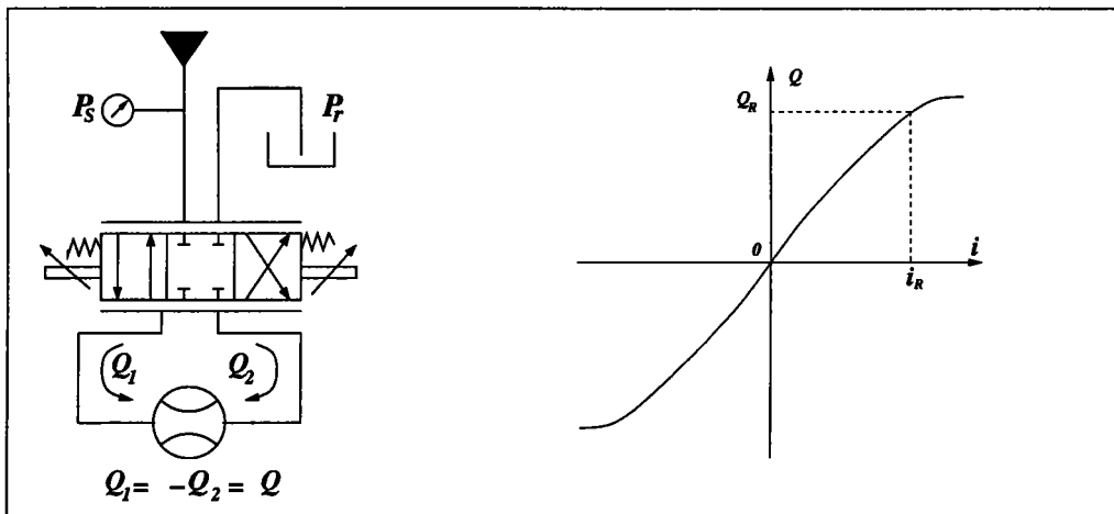
FIG. 2.6 – (a) Setup of the control flow measurement. (b) Flow curve
