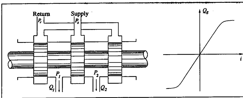
FIG. 2.5 – Critical center spool valve
