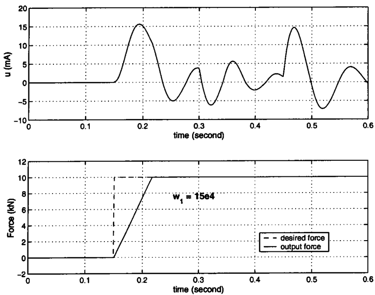
FIG. 3.7 – Force behaviour and needed control law. (tracking constant force)
