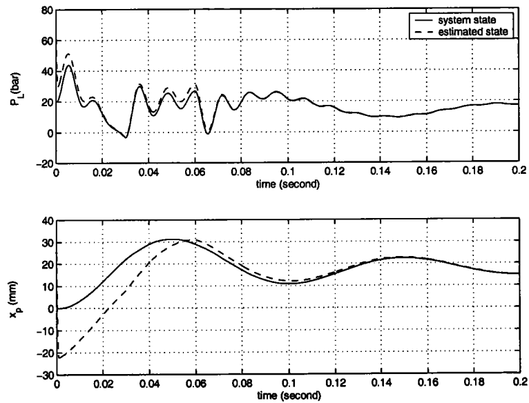
FIG. 5.8 – The sliding observer states robustness to stiffness variations.
