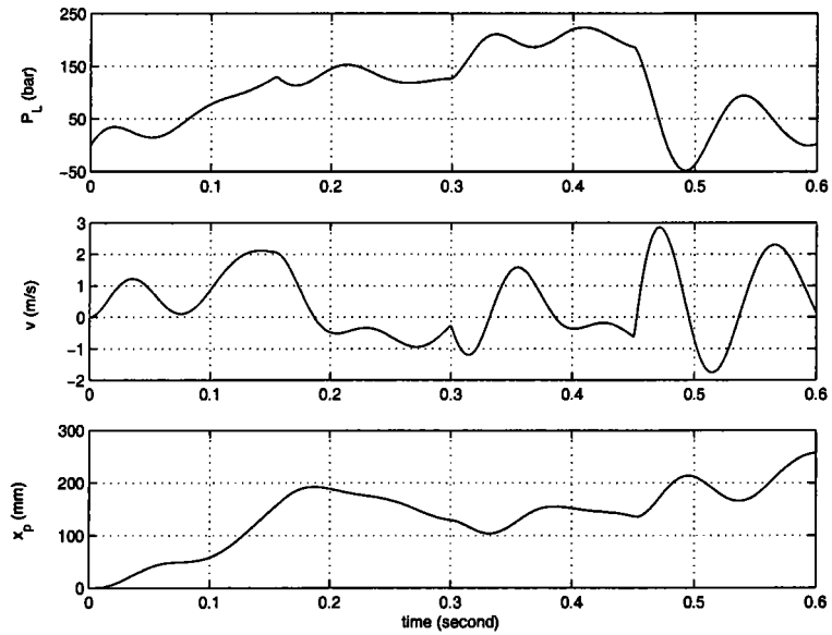
FIG. 3.8 – State behaviour of the system. (tracking time-varying force)
