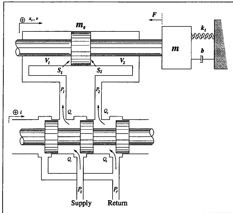
FIG. 2.22 – Valve-piston combination
