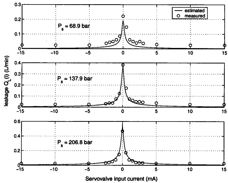
FIG. 2.18 – Measured and estimated internal leakage flow ( Q_L )
