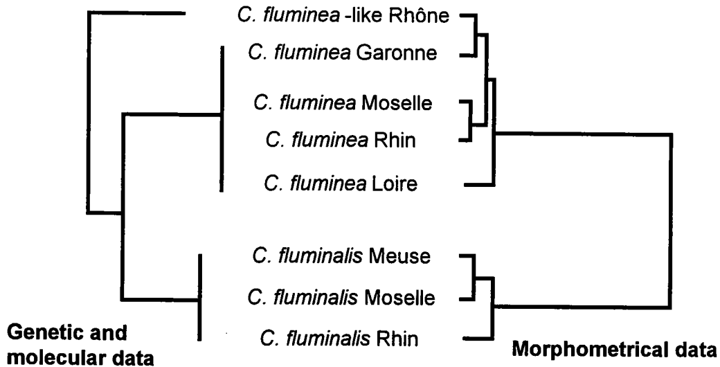
Fig. 3. Diagram illustrating the relationships among Corbicula species. Both topologies indicate significant differentiation for morphometry, nuclear and mitochondrial genomes of C. fluminea and C. fluminalis . The C. fluminea -like population from the Rhône is as much genetically differentiated as the two other species, but morphologically, it falls in the range of variation of C. fluminea .
