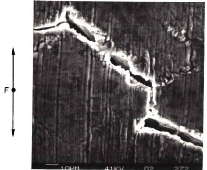
d - Éprouvette N2R50 - Fatigue-relaxation, t_m = 90 min
