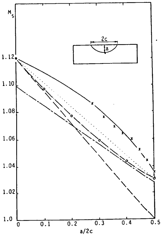
Figure (29) : Différentes valeurs de M_s , selon : — x — SMITH and ALARVI [1] and THRESHER [2] ..... Equation (13) [3] ----- KOBAYASHI and MOSS [4] ----- PARIS and SIH [5] ----- SMITH [6]
