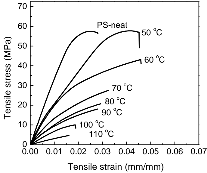
Fig. 5.3 Stress-strain curves for PS foams with various foaming temperatures.
