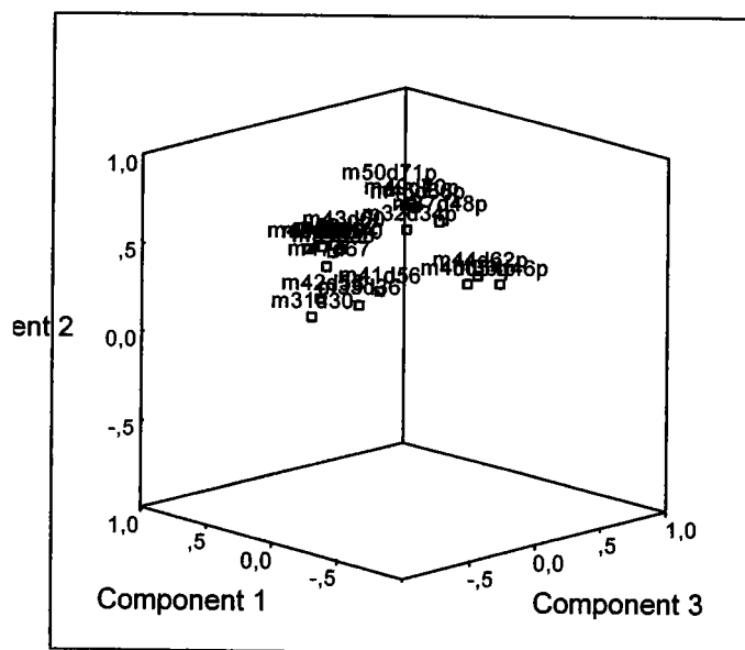
Component Plot in Rotated Space
