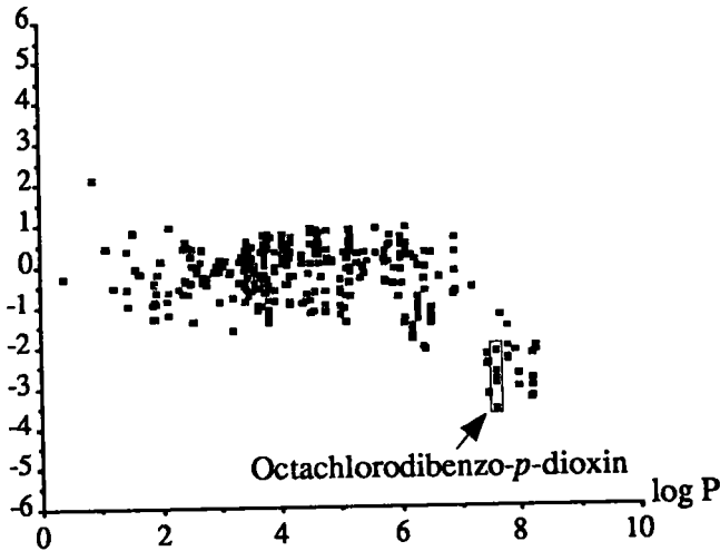
Figure 3 Residuals of Eq. (2) vs log P for BCF data obtained under flow-through conditions.
