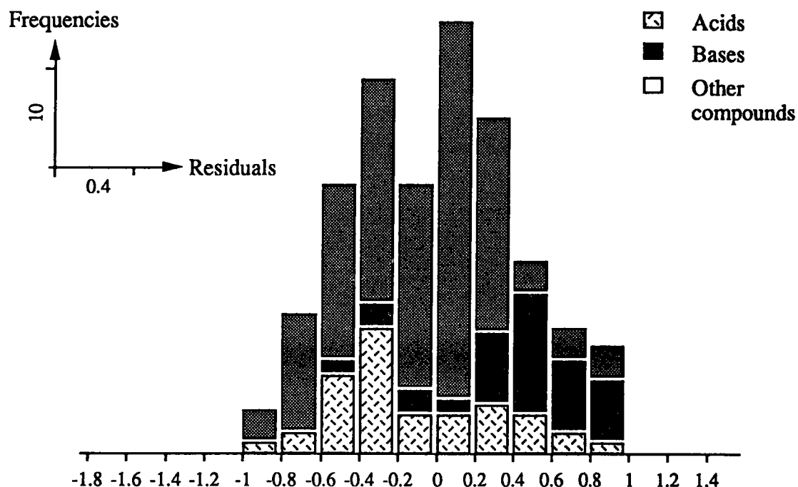
Fig. 4. Graphical analysis of the residuals ( \log K_p \text{ obs.} - \log K_p \text{ calc.} ) obtained with Eq. 9.
