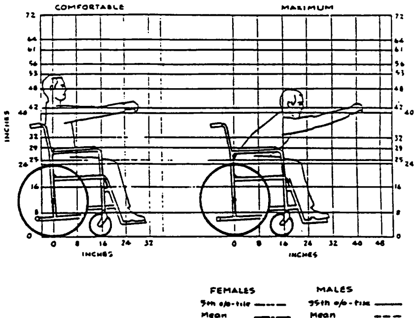
FORWARD REACH (Adults)
