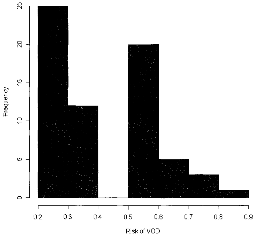
Figure 1: Distribution of patients' preconditioning risk score of veno occlusive disease (VOD). The risk score was estimated as proposed by Baker et al (21)
