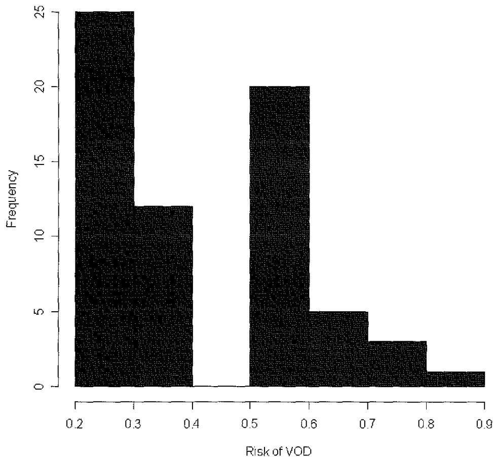
Distribution of VOD risk score
