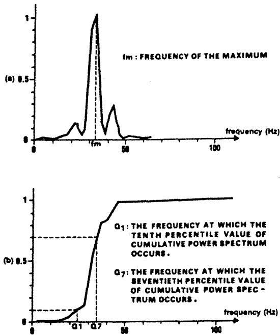
FIG. 6. Seismic variables computed from power spectrum.
