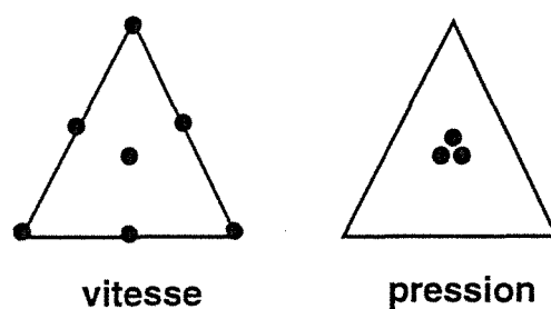
Figure 4.2 Élément fini P_2^+ - P_1 .
