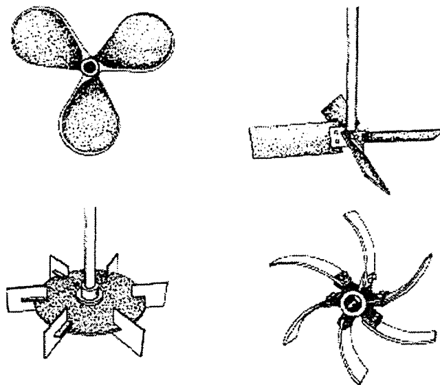
Figure 1.1 Turbines (haut:type axial ; bas:type radial).
