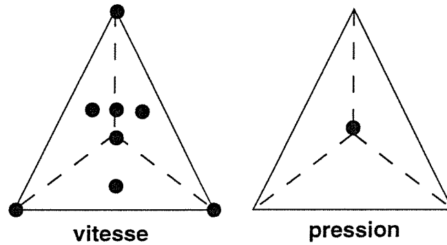
Figure 2.2 élément fini P_1^+ - P_0 .
