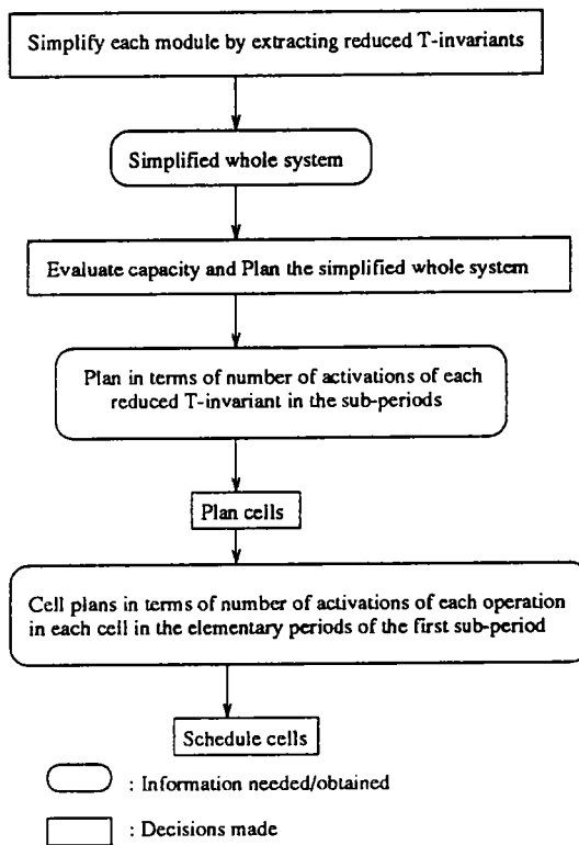
FIG. C.15 - Hierarchical planning
