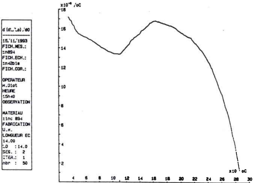
Courbe d(dL/L_0)/dT = f(T) : alliage 31894
