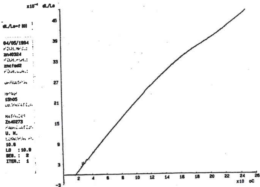
Courbe dL/L_0 = f(T) : alliage 40324
