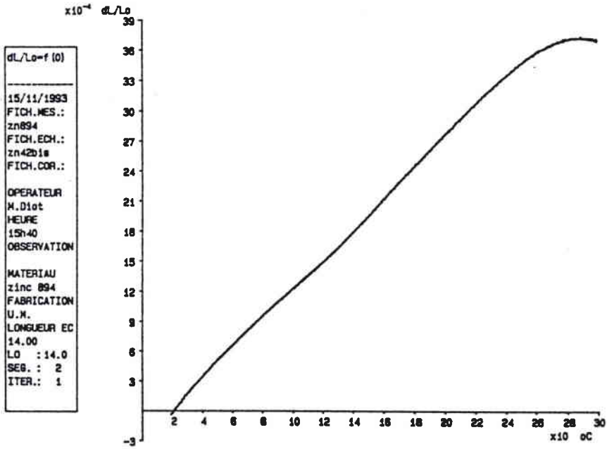
Courbe dL/L_0 = f(T) : alliage 31894
