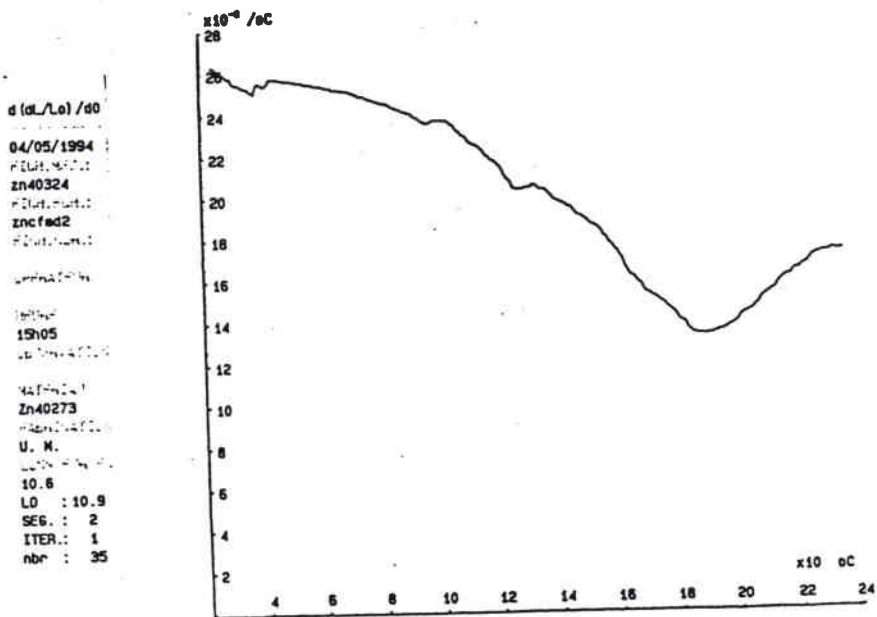
Courbe d(\text{dL/L}_0) / dT = f(T) : alliage 40324
