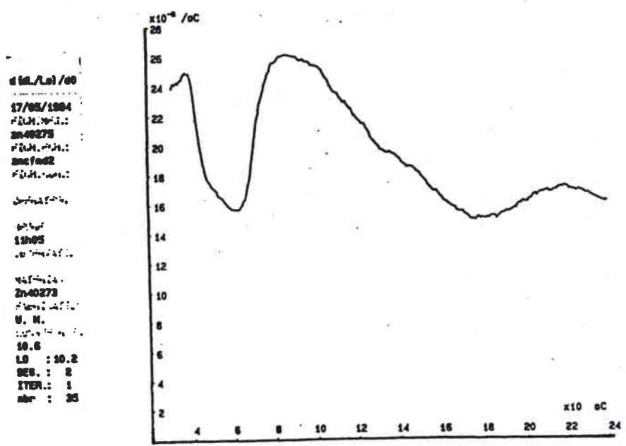
Courbe \frac{d(dL/L_0)}{dT} = f(T) : alliage 40275
