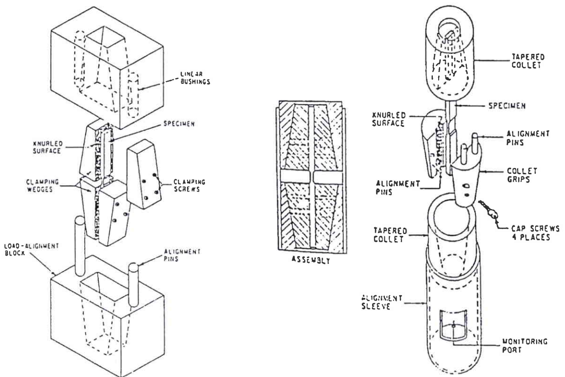
Figure A 10 : Montages IITRI (Illinois Institute of Technology and Research Institute) et Celanese (Corporation).
